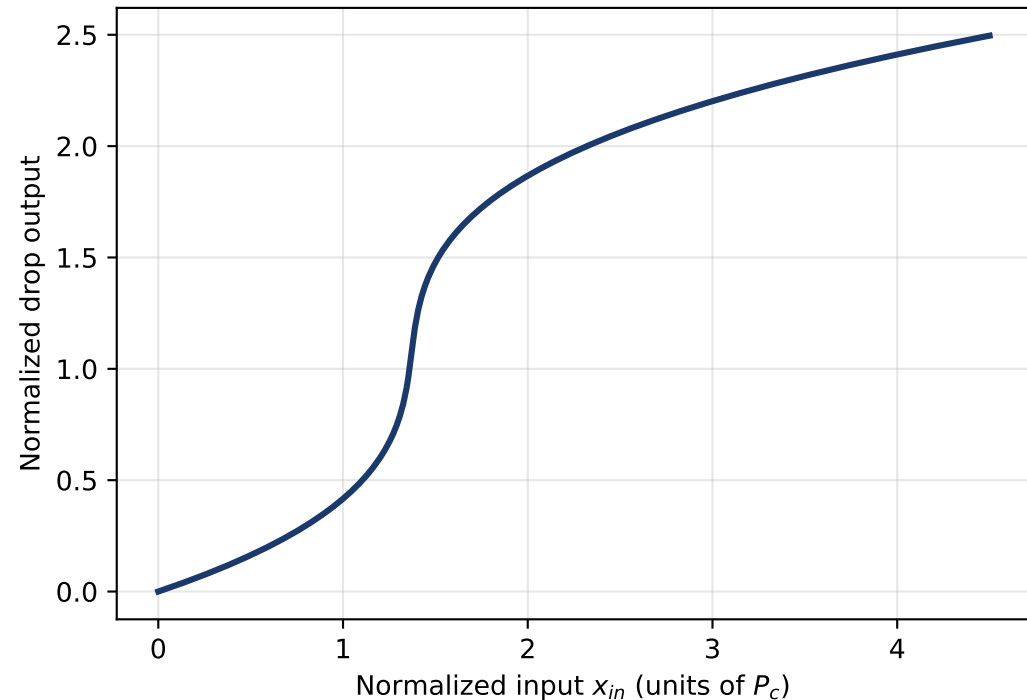
Kerr microring transfer ( \Delta=1.6 , below bistability)
