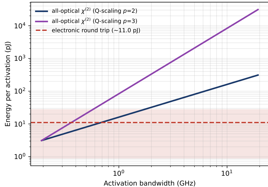
Energy/op: all-optical vs electronic
