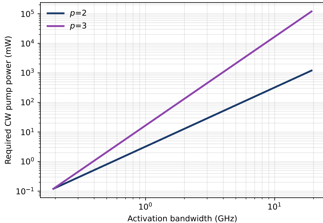
Pump power for 30% conversion
