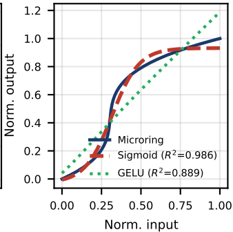
Fit to activations
