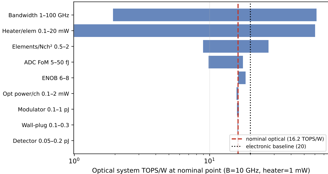
Sensitivity of optical TOPS/W (tornado)
