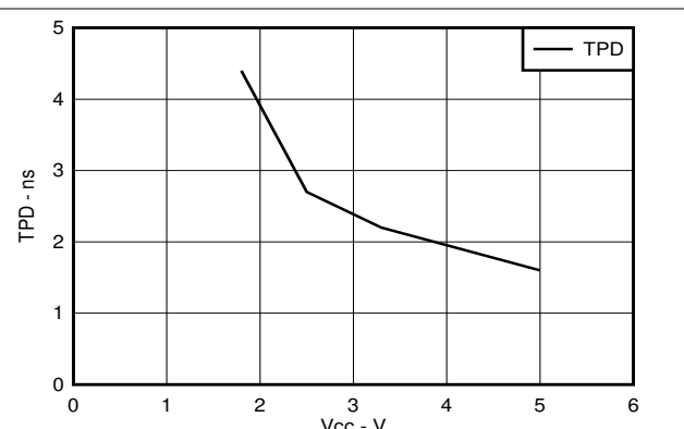
Figure 5-2. TPD Across V_{CC} at 25°C
