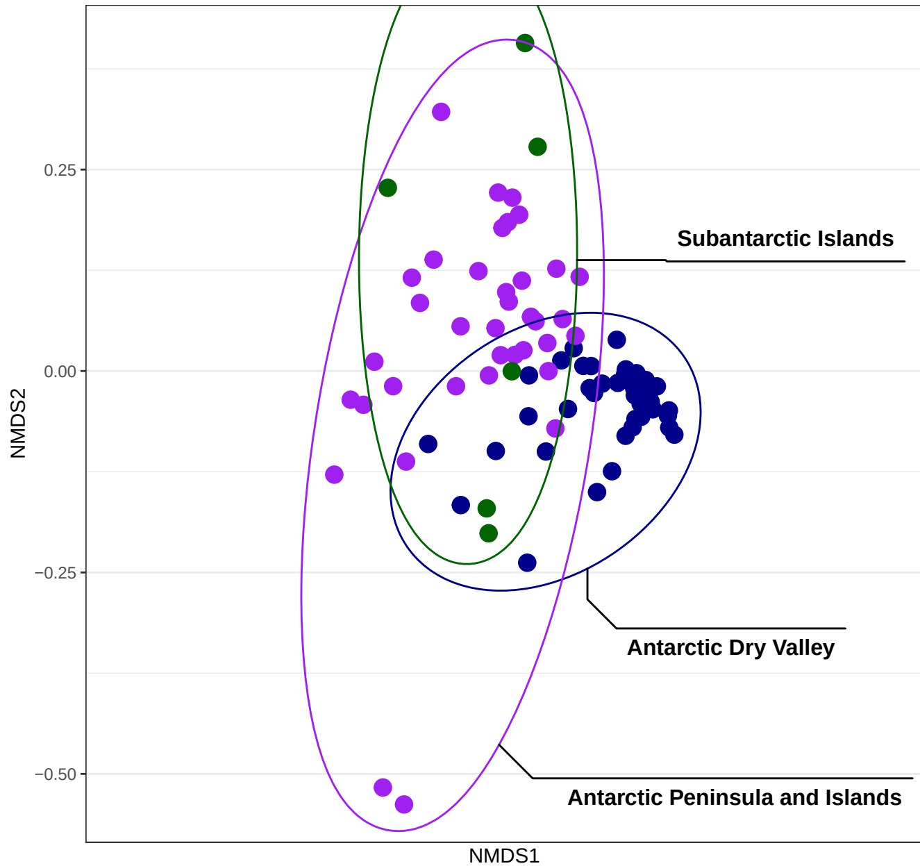
Family NMDS
