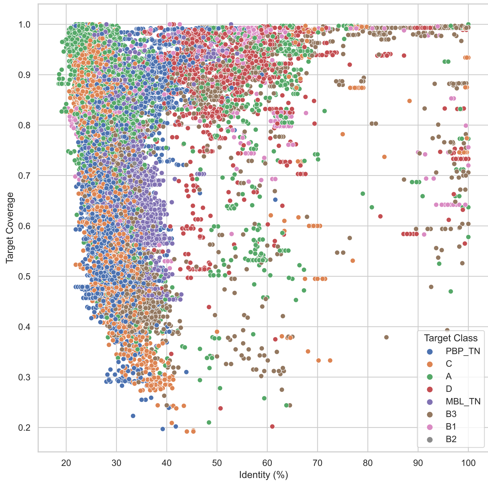
Potential BLAs
