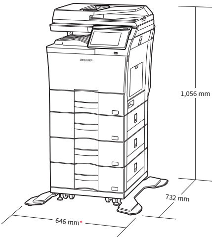
* 736 mm when the Anti-tip Kit for Stand is attached and the multi bypass tray is extended. Shown with optional equipment.
