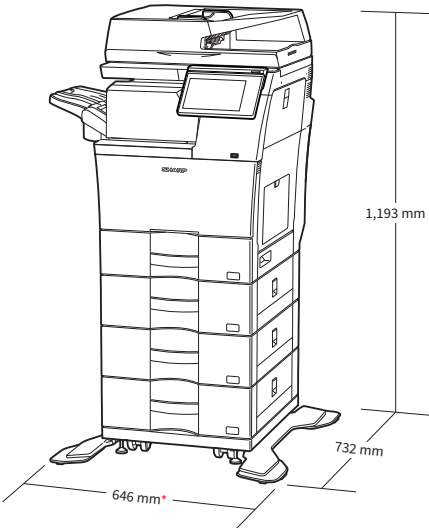
* 872 mm when the finisher tray and multi bypass tray are extended. Shown with optional equipment.
