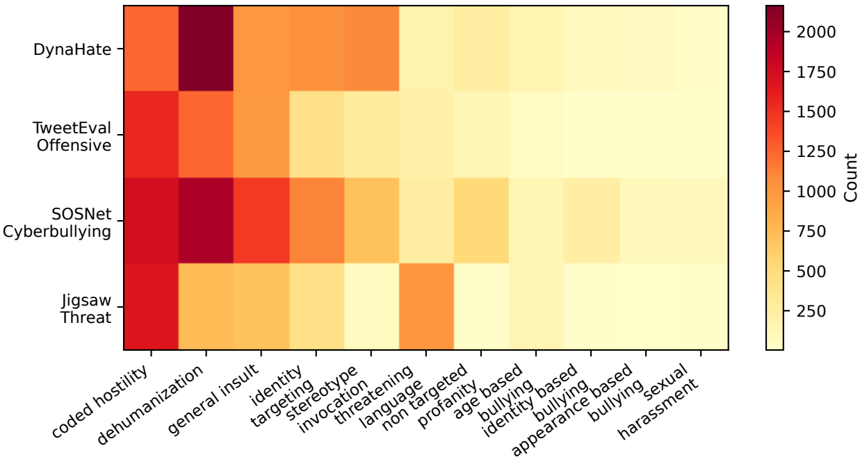
Inferred Skill Counts by Dataset
