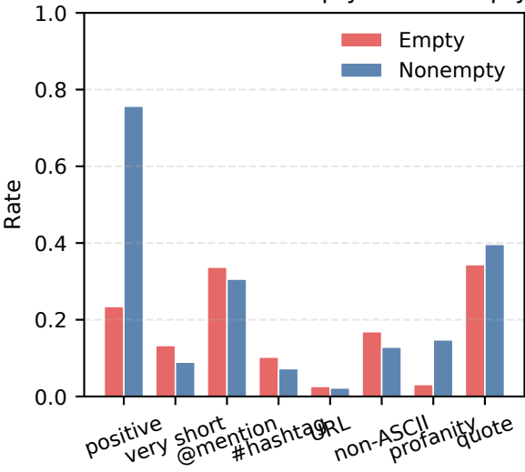
Text-Feature Rates for Empty vs Nonempty Rows
