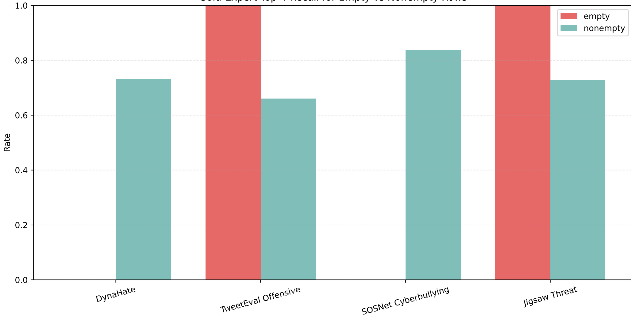
Gold-Expert Top-4 Recall for Empty vs Nonempty Rows
