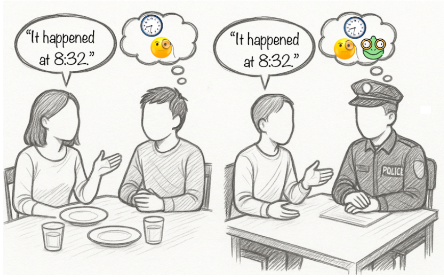
(c) model predictions for which knowledge states and motivation-based strategies a listener considers as probable after a speaker utters v_{prc} (left: dinner context; right: police context)
