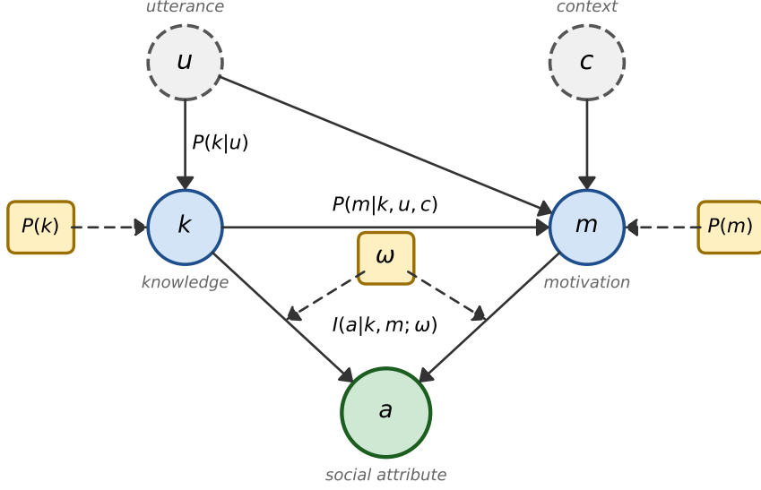
Figure 2: Bayesian network representation of the Social Evaluation Model. Dashed circles denote observed variables (utterance u , context c ) available to the listener. Solid circles denote latent variables inferred by the listener: knowledge state k , motivation-based strategy m , and evaluation of the social attribute a . Rectangles denote free parameters: prior probabilities P(k) and P(m) , and the weight parameter \omega . Inference proceeds in three stages: u and P(k) jointly determine the posterior over knowledge states P(k|u) ; k , u , c , and P(m) determine the posterior over strategies P(m|k, u, c) ; and k and m feed into the impact function, weighted by \omega , to yield the social evaluation of attribute a .
