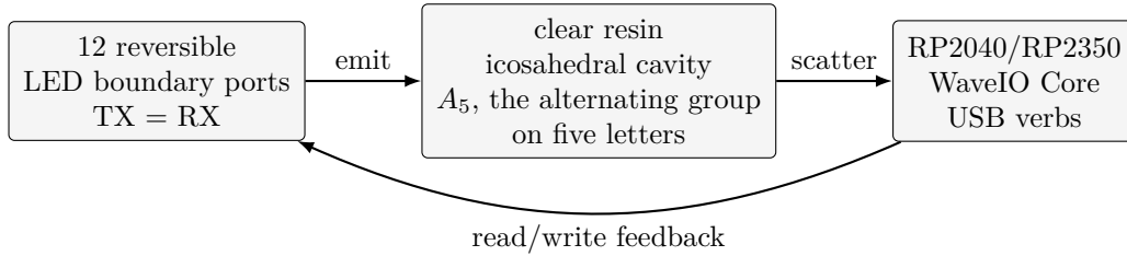
Figure 1: Short version of the Echosahedron as a controllable single-patch hardware instance: a finite boundary, reversible read/write ports, geometric coupling, firmware records, and a designed overlap response.
