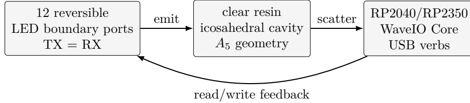
Figure 1: Short version of the Echoshedron as a controllable single-patch hardware instance: a finite boundary, reversible read/write ports, geometric coupling, firmware records, and measured overlap response.
