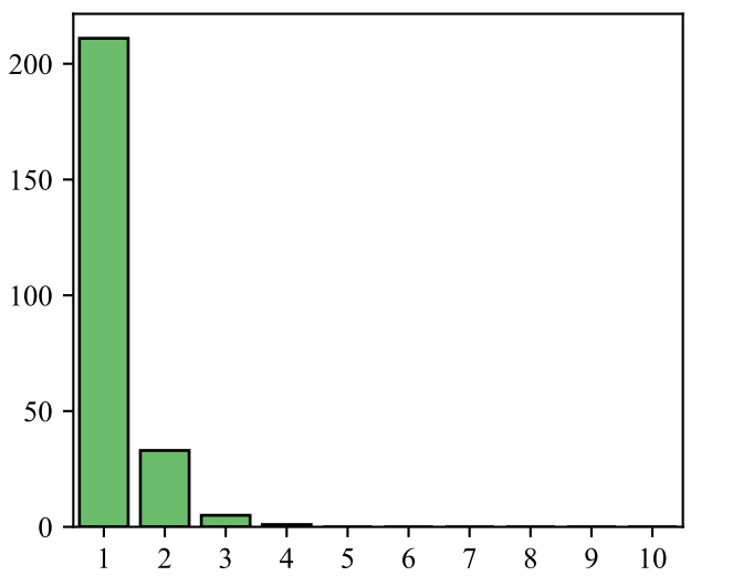
DeepSeek-Llama-70B
