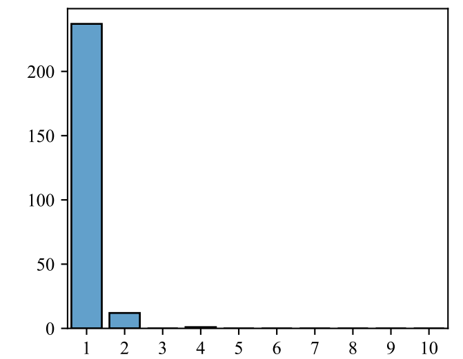
Mistral-Small-3.2-24B
