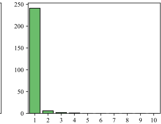
gpt-oss-120b
