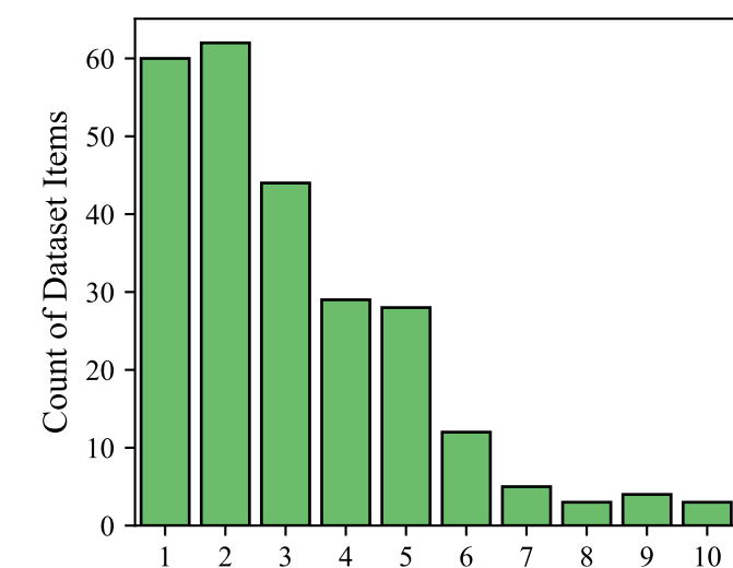
SciBench
