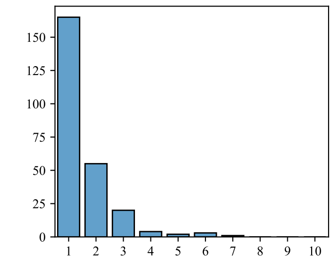
Ministral-8B
