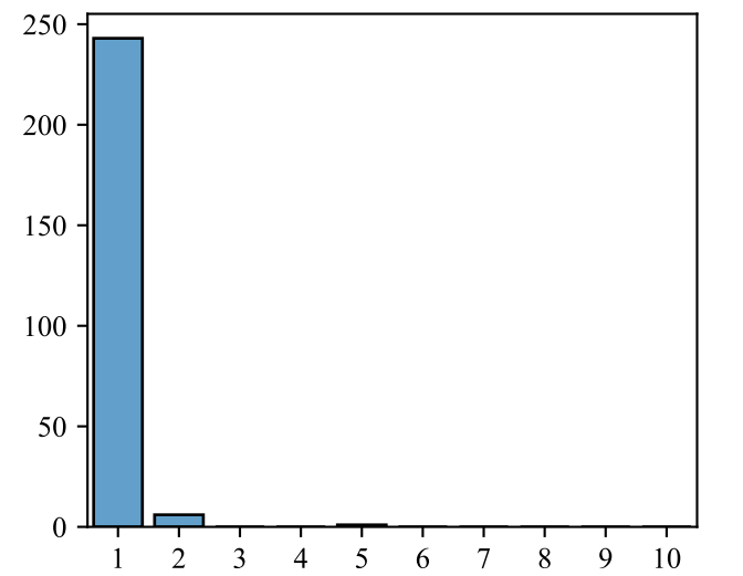
Qwen3-30B-A3B-Instruct
