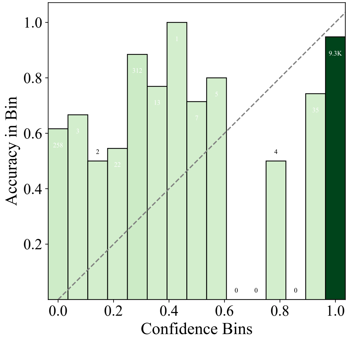
Verbalized Uncertainty
