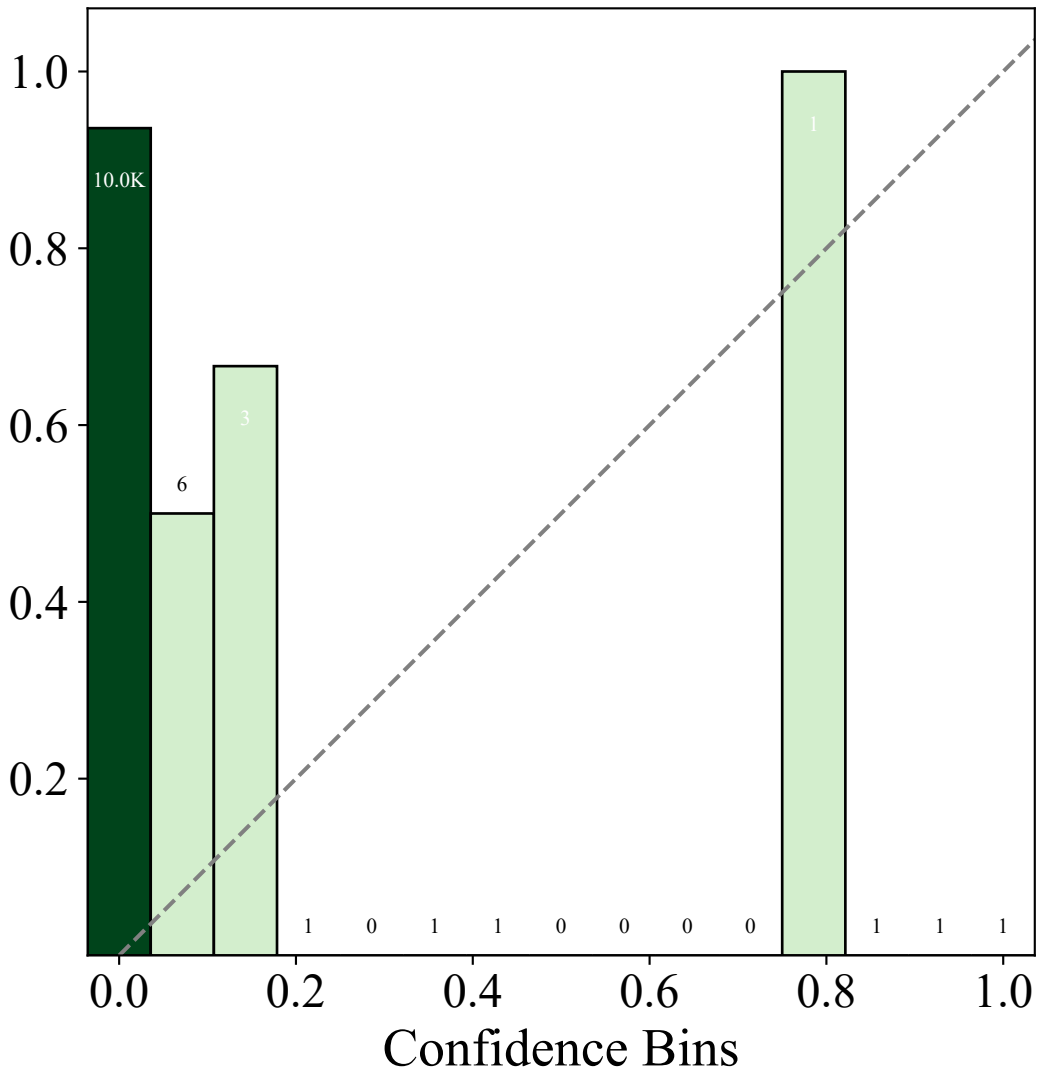
CCP
