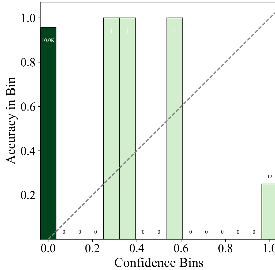
CCP
