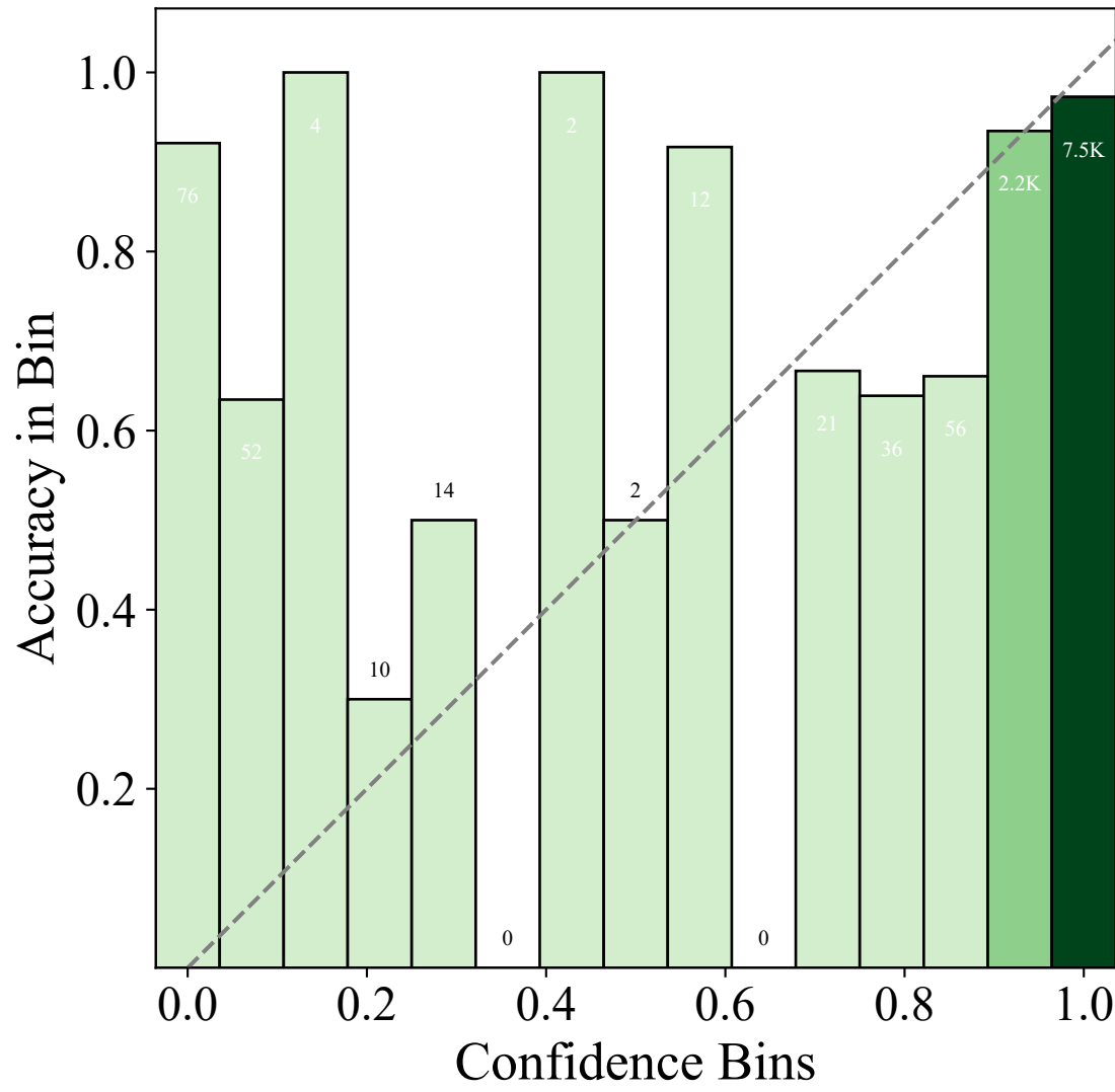
Verbalized Uncertainty
