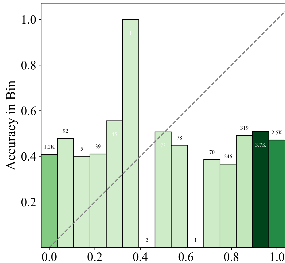
Verbalized Uncertainty
