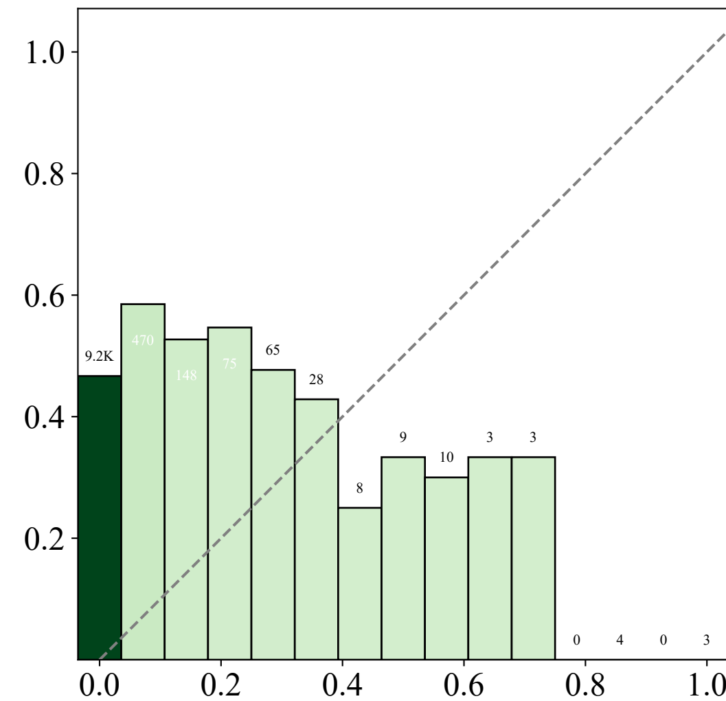
CCP
