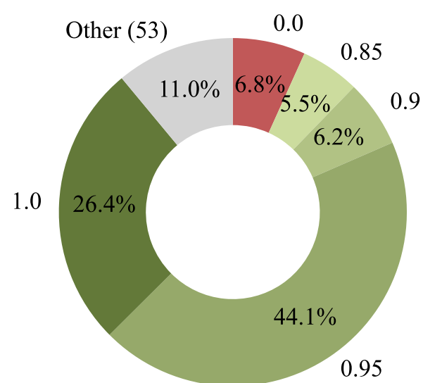
Magistral-Small-24B-Reasoning
