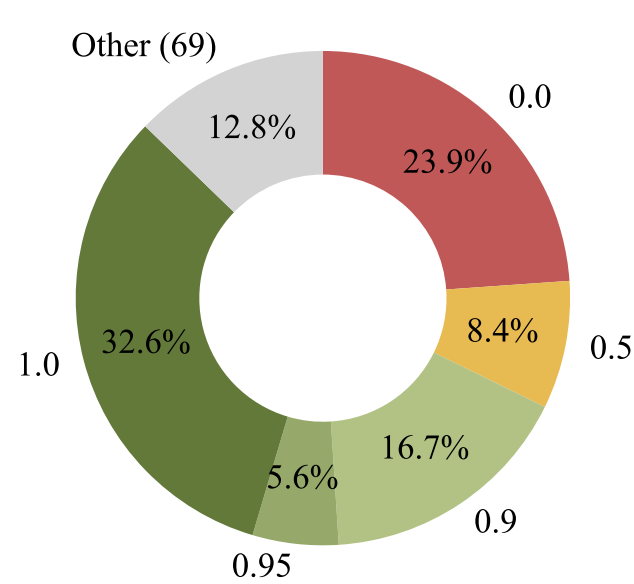
Ministral-8B
