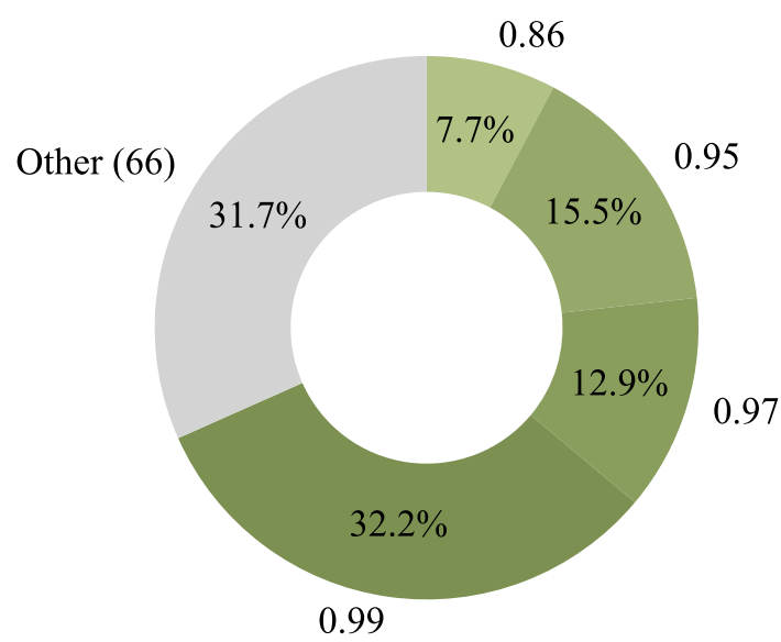
gpt-oss-120b
