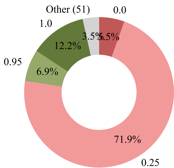
Qwen3-30B-A3B-Instruct
