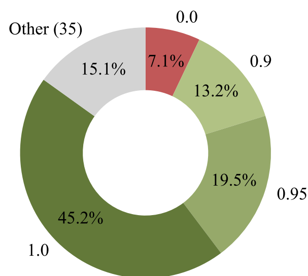
Mistral-Small-3.2-24B
