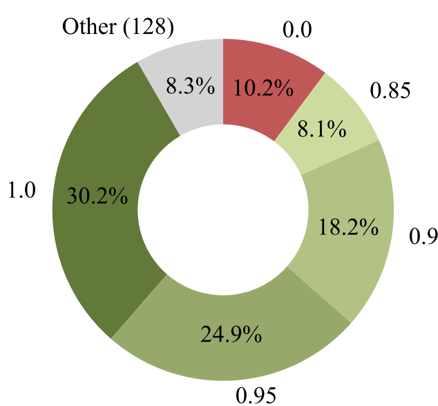
DeepSeek-Llama-70B
