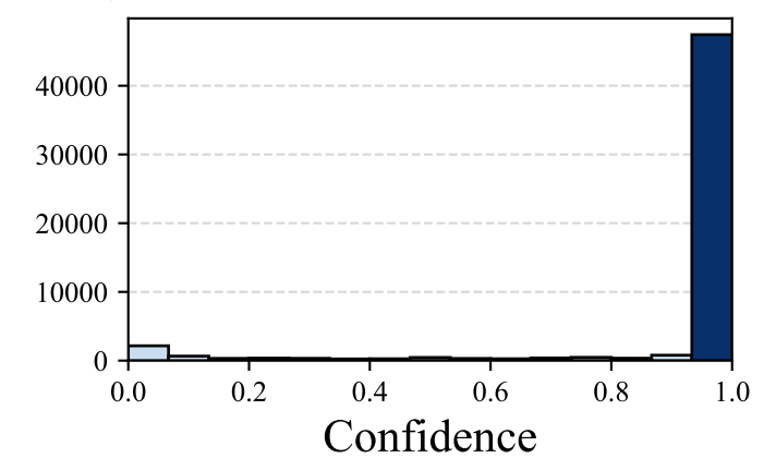
Qwen3-30B-A3B-Instruct-2507
