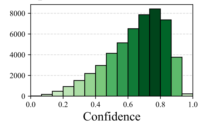
DeepSeek-R1-Distill-Llama-70B
