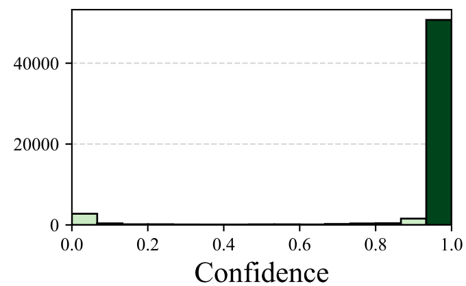
gpt-oss-120b
