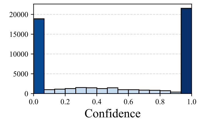
Mistral-Nemo-Instruct-2407
