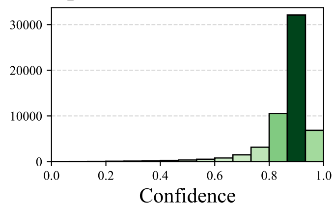
DeepSeek-R1-Distill-Qwen-32B
