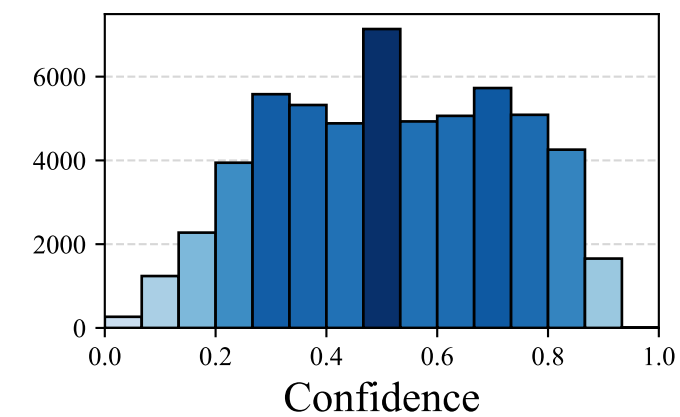
Ministral-8B-Instruct-2410
