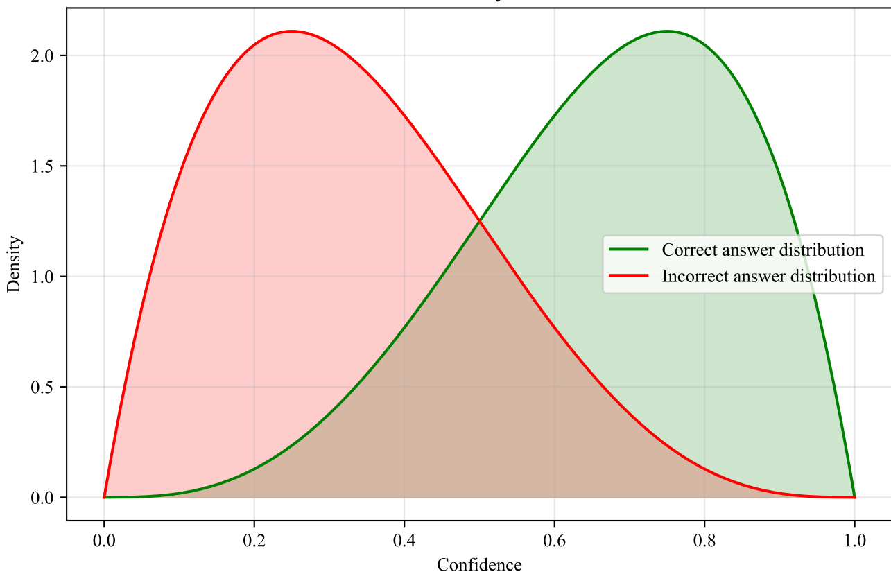
Beta Distributions for Synthetic Confidence
