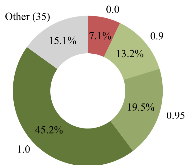
Mistral-Small-3.2-24B
