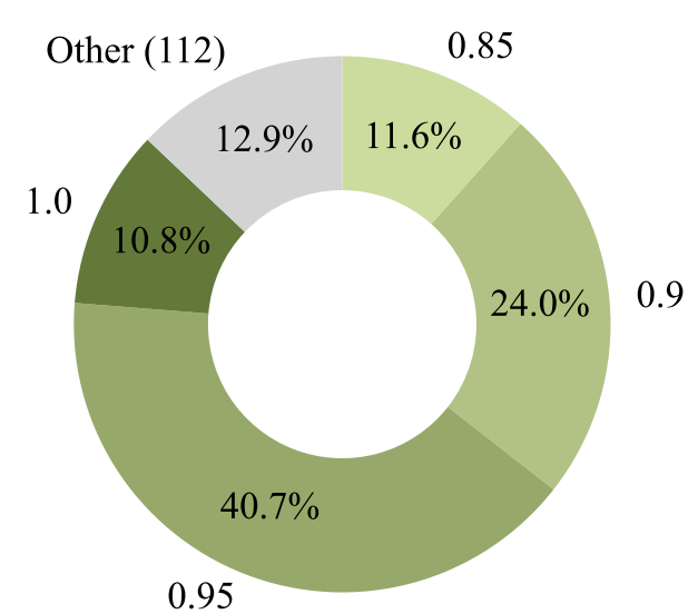
DeepSeek-Llama-70B
