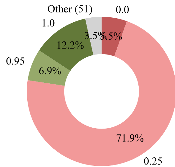
Qwen3-30B-A3B-Instruct
