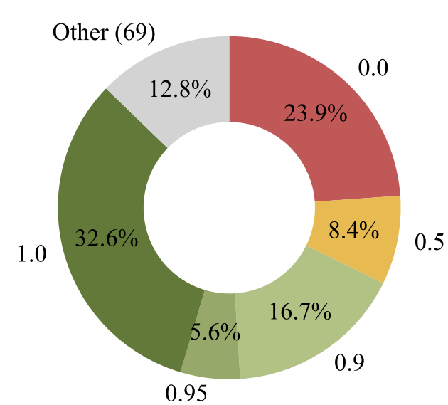
Ministral-8B
