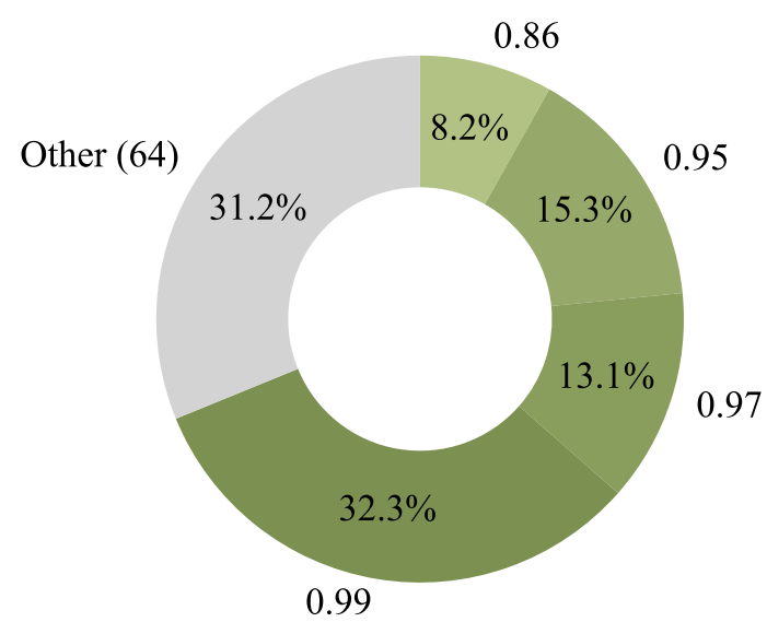
gpt-oss-120b
