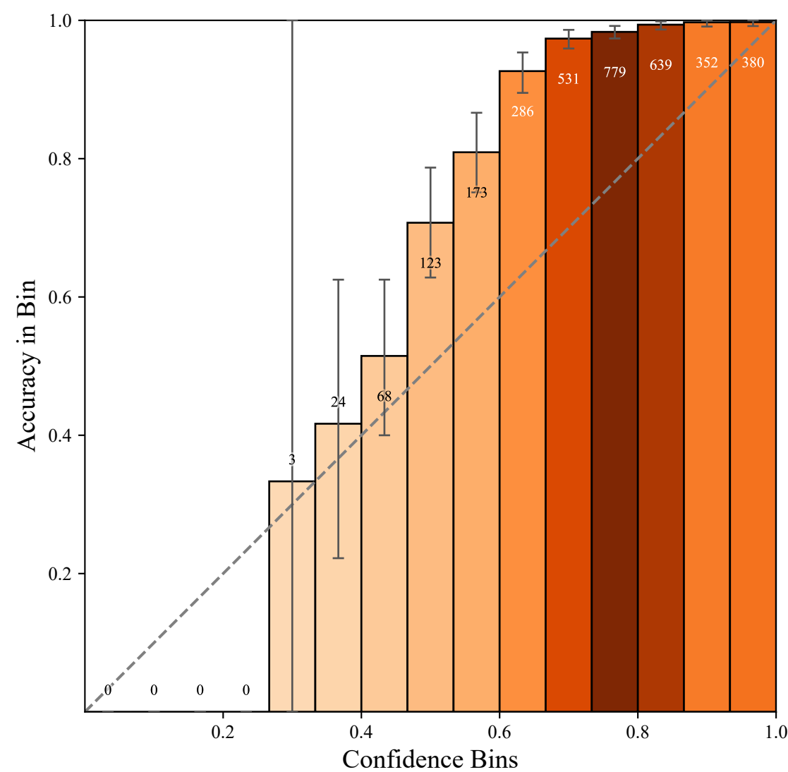
ArcReasoning
