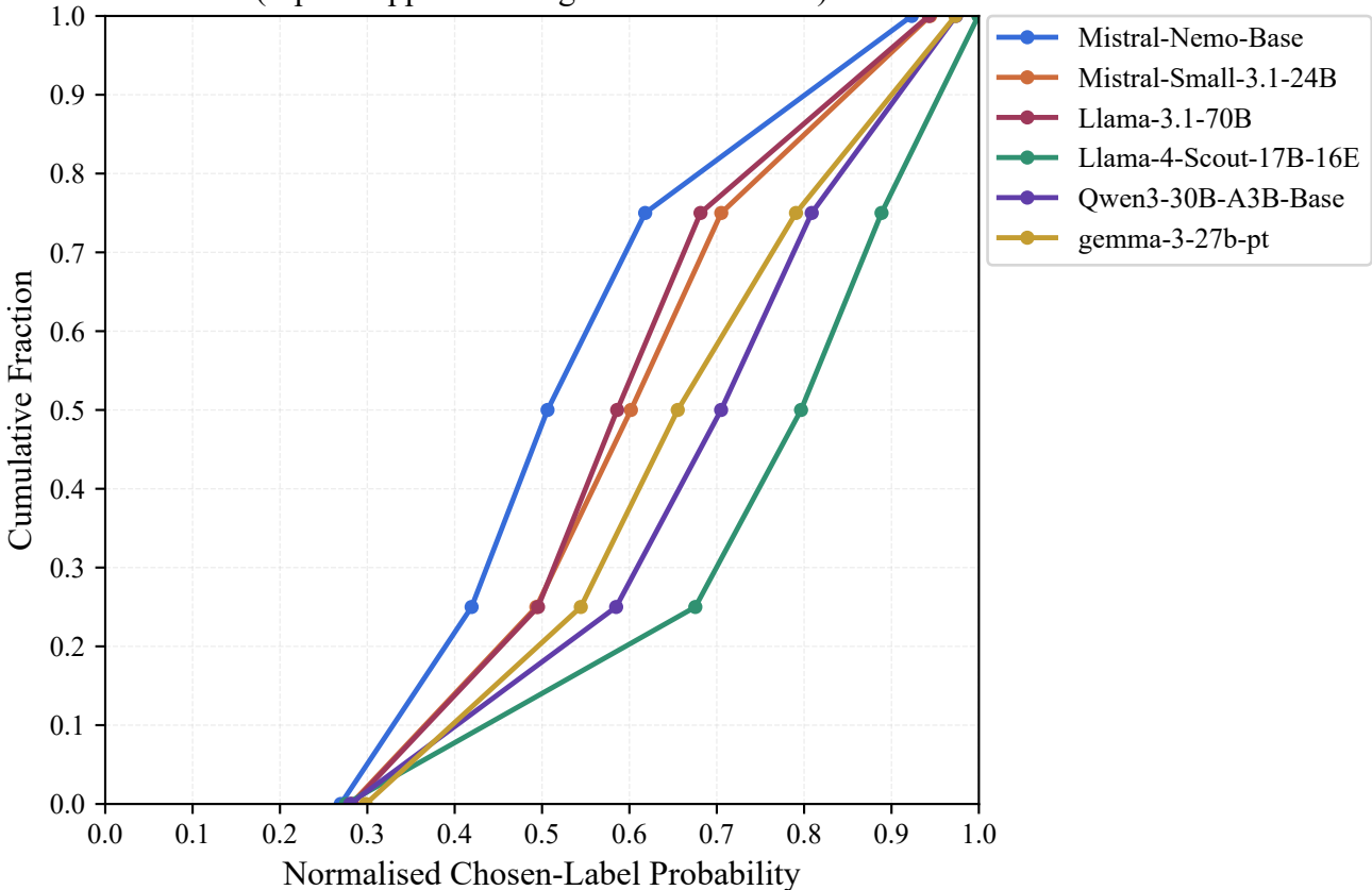
ECDF of Uncertainty Scores — Base Models (5-point approx. averaged across datasets)
