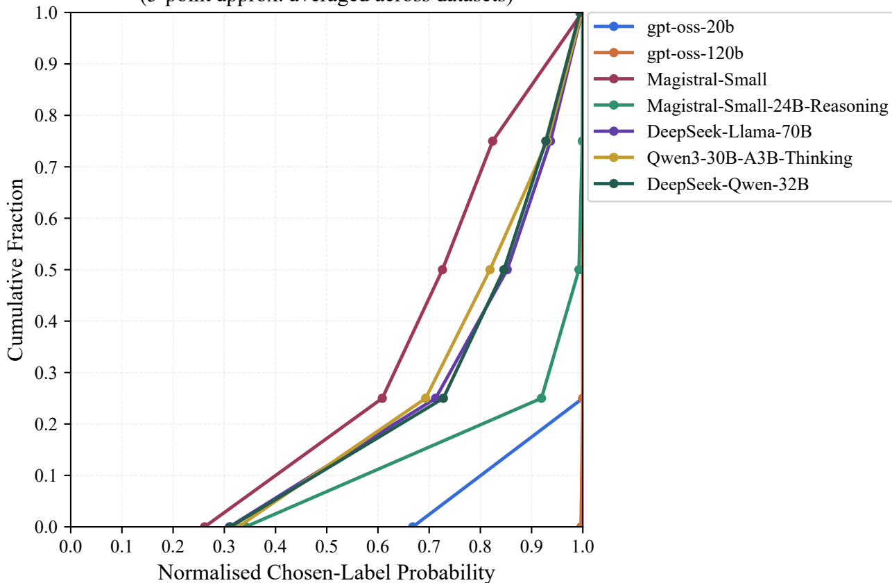
ECDF of Uncertainty Scores — Reasoning Models (5-point approx. averaged across datasets)
