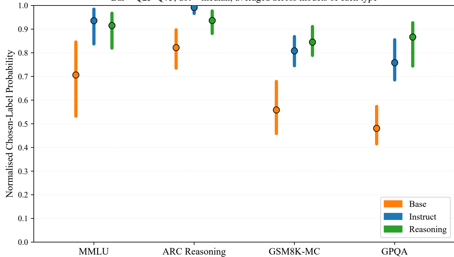
IQR per Model Type per Dataset (norm_chosen) Bar = Q25–Q75, dot = median; averaged across models of each type
