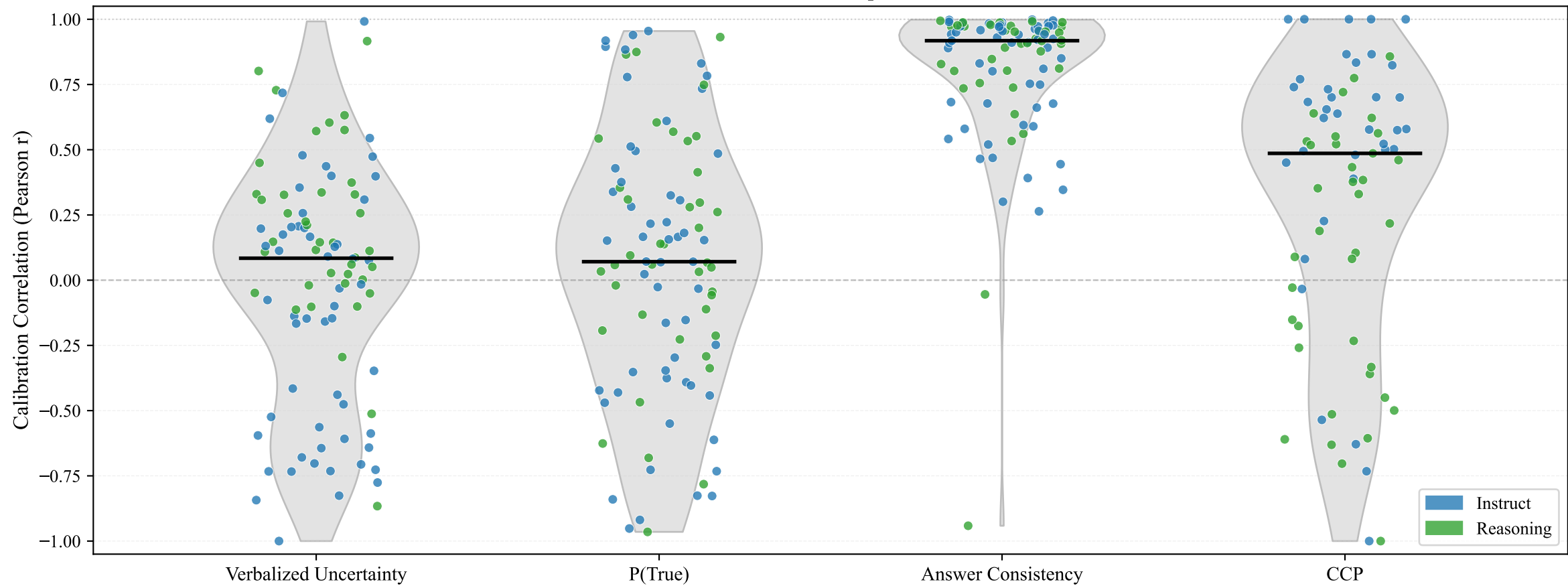
Calibration Correlation per UQ Method
