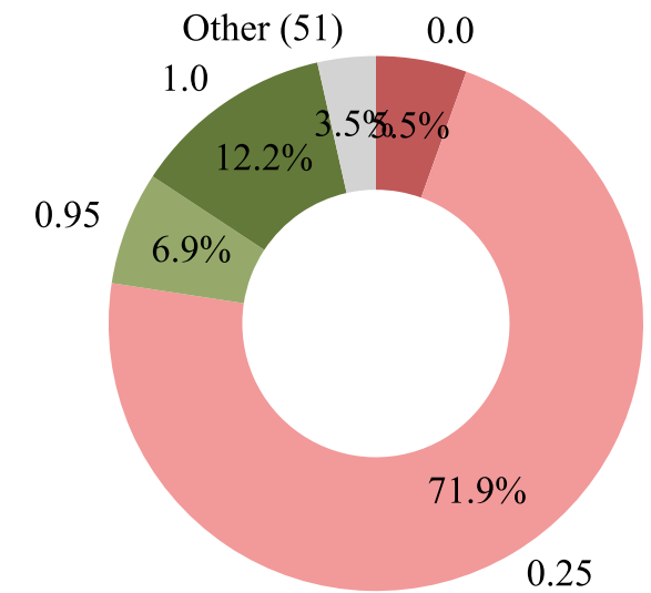
Qwen3-30B-A3B-Instruct
