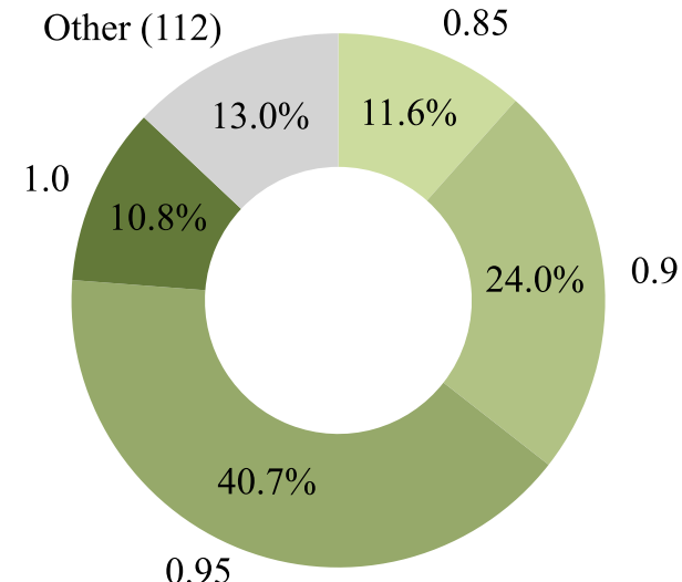
DeepSeek-Llama-70B
