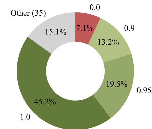
Mistral-Small-3.2-24B
