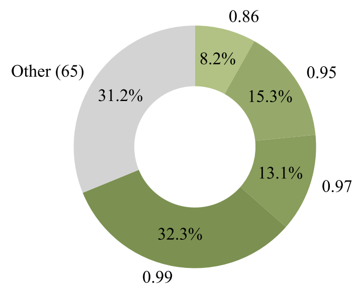
gpt-oss-120b
