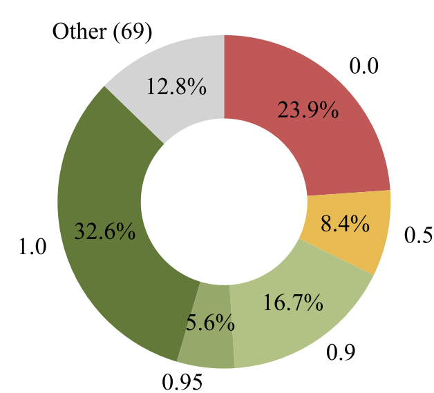
Ministral-8B
