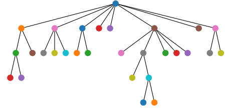
Figure 2: Top: An example octree constructed in three-dimensional space to partition twenty points, constructed with an arbitrary insertion order. Bottom: The same octree, represented two-dimensionally.
