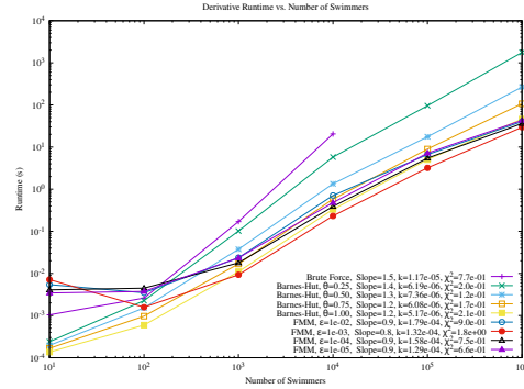
Figure 3: A logarithmic-scale runtime comparison plot for each derivative computation method when parallelized using an eight-core CPU.
