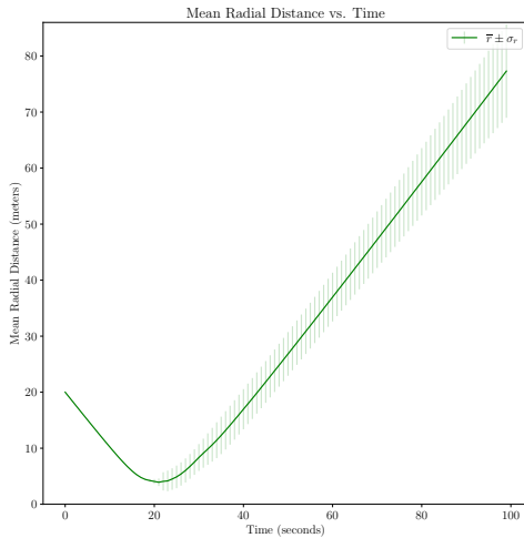
Figure 7: The mean and standard deviation of radial distance as a function of time for the implosion example.
