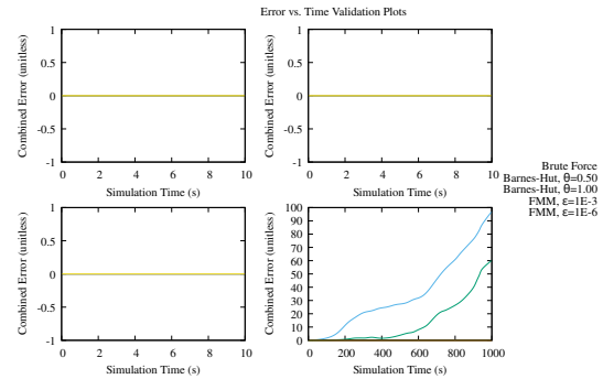
Figure 5: The numerical validation comparison plots of the error in the simulation versus the time. The top left, top right, and bottom left plots are two-swimmer, coplanar simulations. The bottom right plot is a 13-swimmer trajectory from Figure 9(b) of Mabrouk and Floryan 2025 [4].
