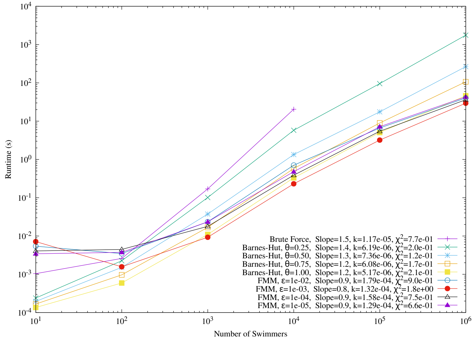
Derivative Runtime vs. Number of Swimmers
