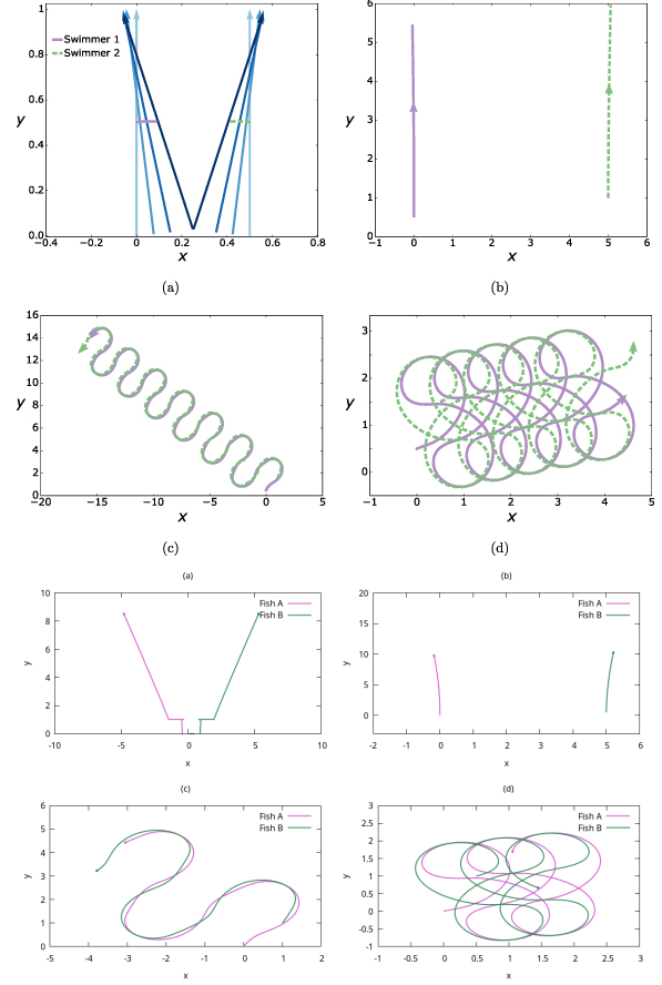
Figure 4: The coplanar, two-swimmer trajectory plots shown in figure 8 of Mabrouk and Floryan 2025 (top) and its reproduction with FINDS (bottom). Note that the two simulations need not exactly match in time as the observed behavior in each case is stable, thus only a few repetitions are necessary to observe similar behavior. Additionally, figure (a) matches the correct behavior, as the original figure was simply conveying the growing separation between the two swimmers over time.
