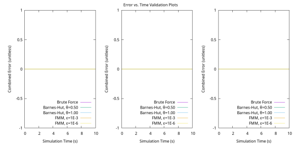
Figure 5: The numerical validation comparison plots of the error in the simulation versus the time, where the first three plots are 2-dimensional, 2-swimmer coplanar comparisons.
