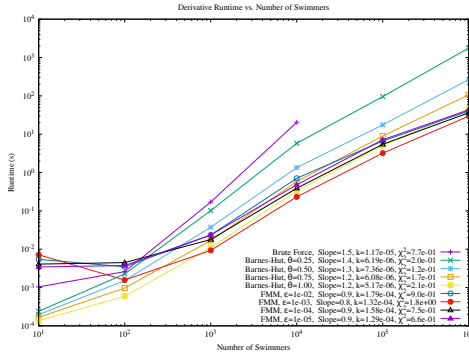
Figure 3: A runtime comparison plot for each derivative computation method.
