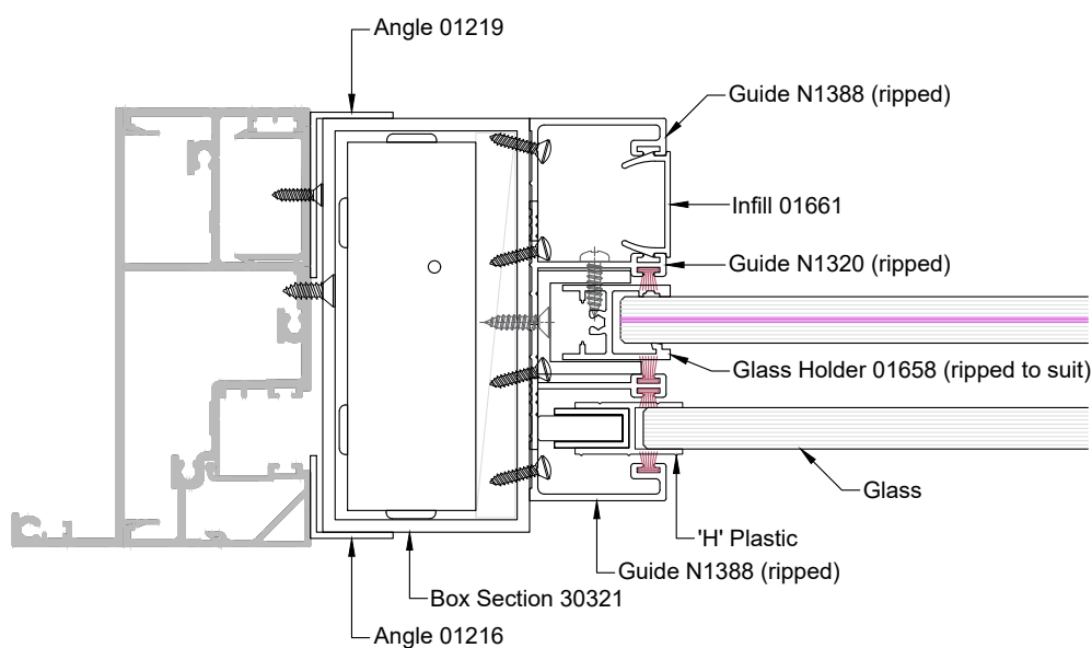
SECTION B-B
