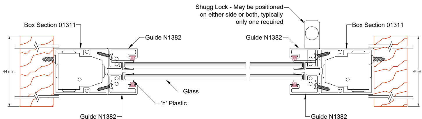
SECTION B-B
