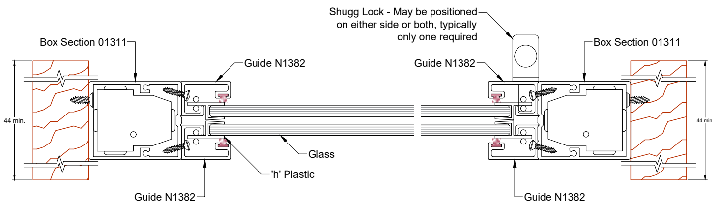
SECTION B-B
