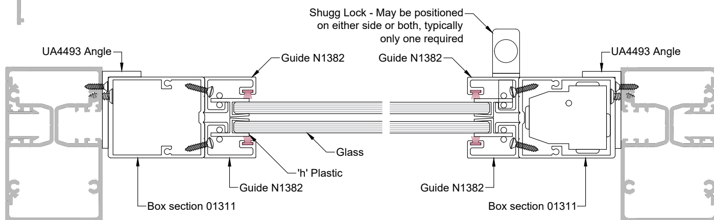
SECTION B-B
