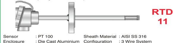
Product Name: RTD Assembly With Adjustable Tri-Clamp Connection
