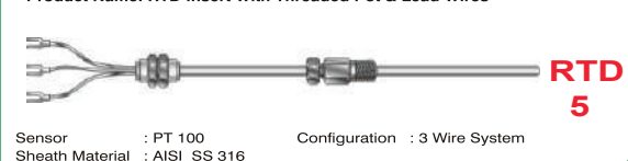
Product Name: RTD Insert With Threaded Pot & Lead Wires
