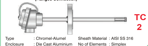
Product Name: TC Assembly With Protecting Tube (Flanged Connection)
