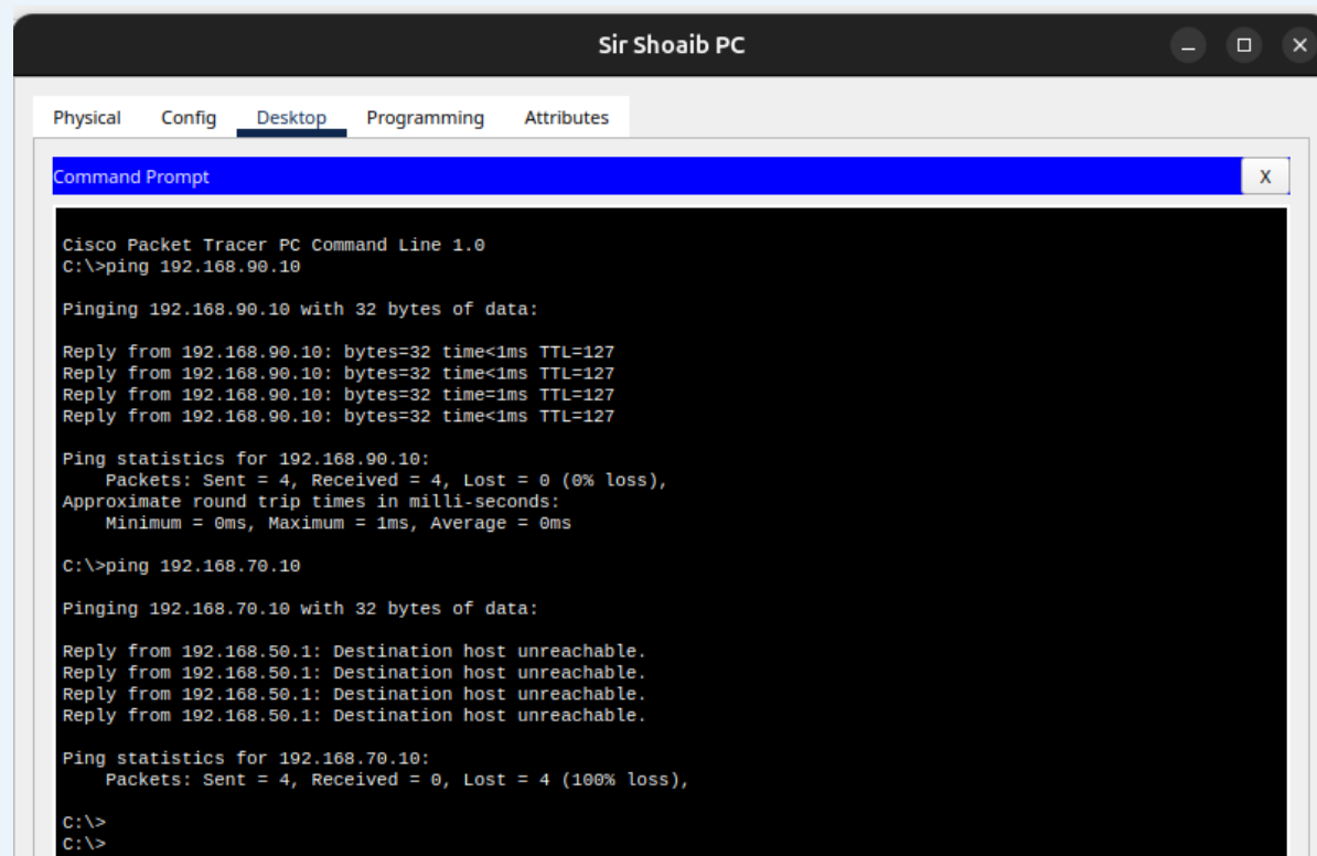
Faculty Member Pings to HOD (Success) & Exam (Fails)
