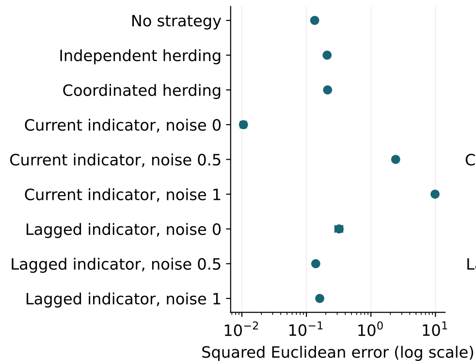
A Mean error
