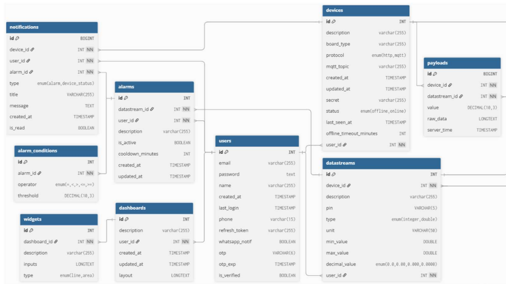
Gambar 3.6 Entity Relationship Diagram
