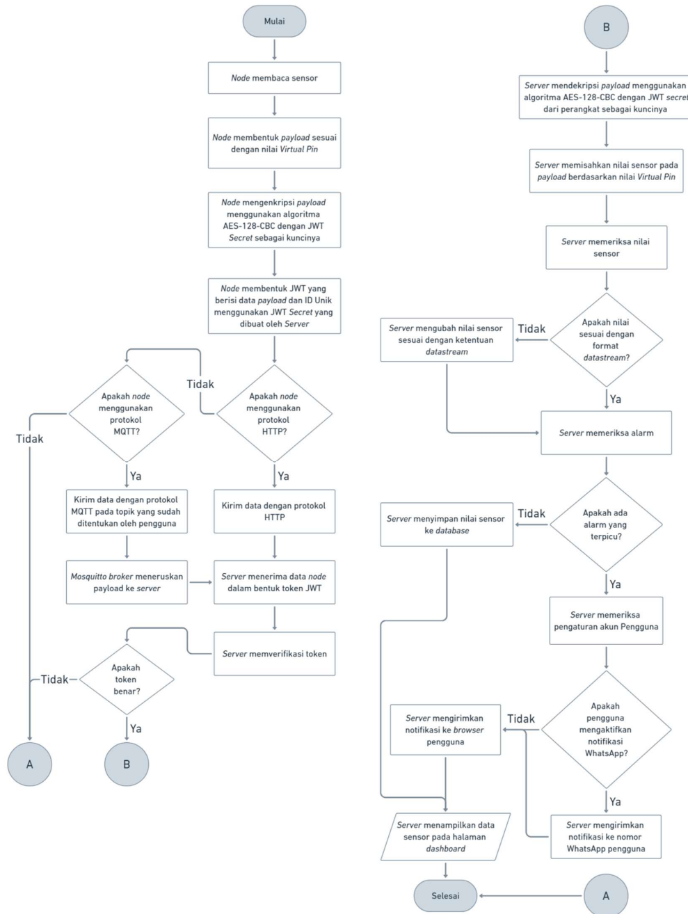
Gambar 3.9 Diagram alur node
