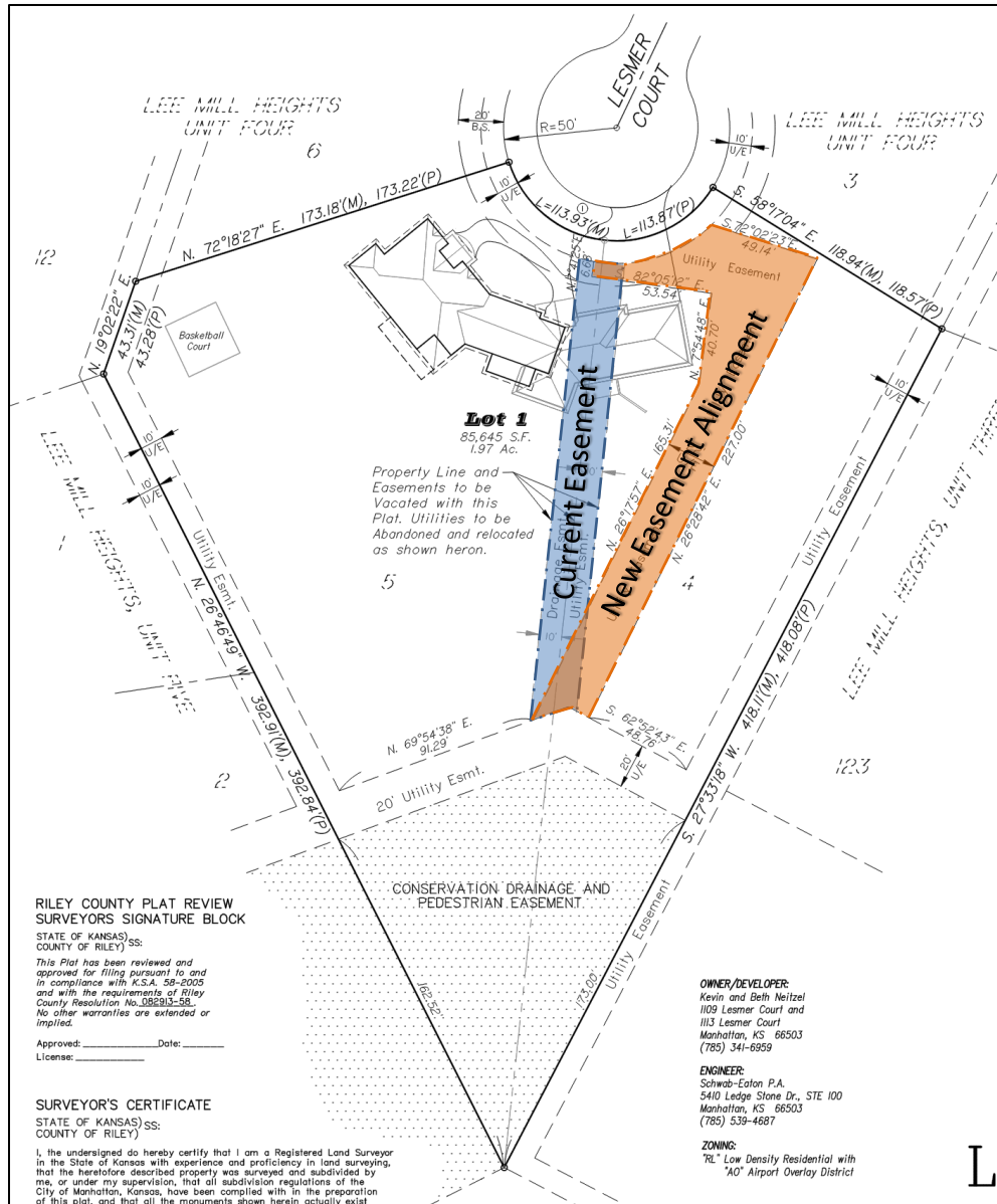
Fig. 2: Lee Mill Heights, Unit 13 – New Easement Alignment
