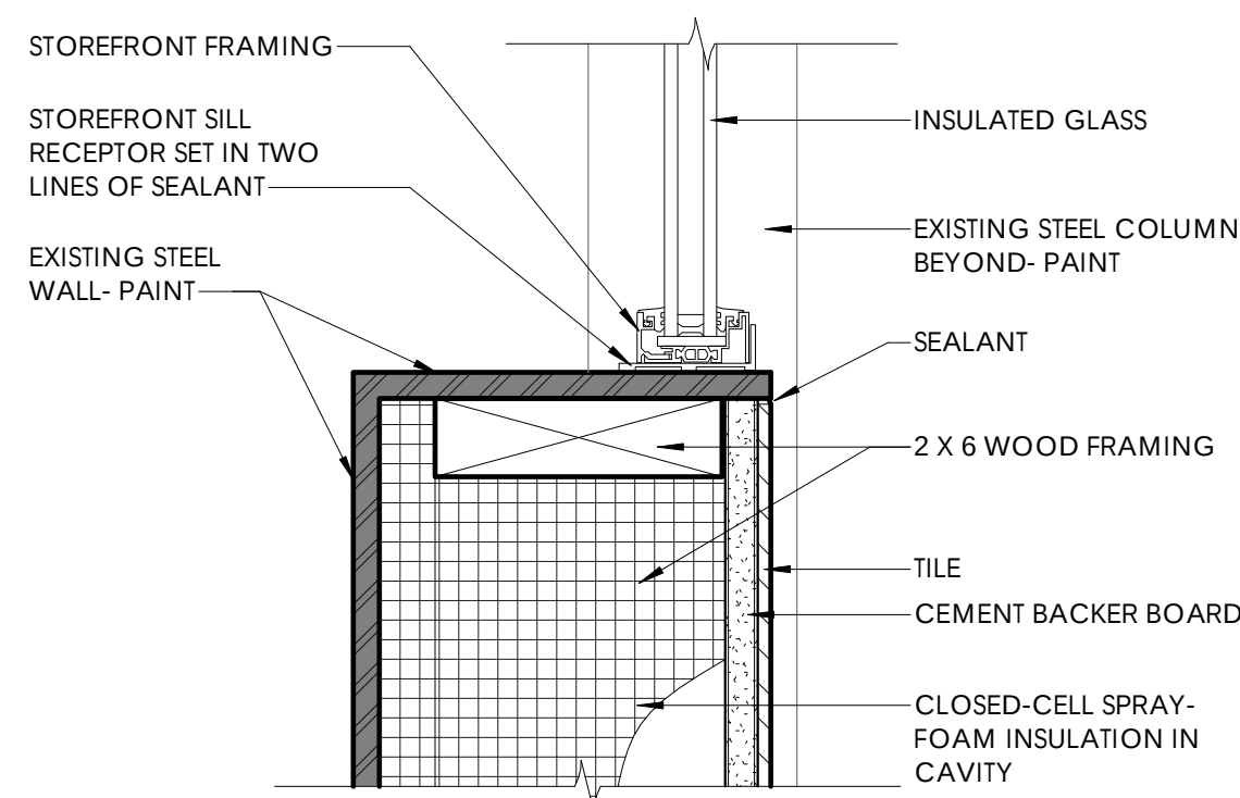
D2 A7.02 LOBBY WINDOW SILL AT KNEE WALL 3" = 1'-0"
