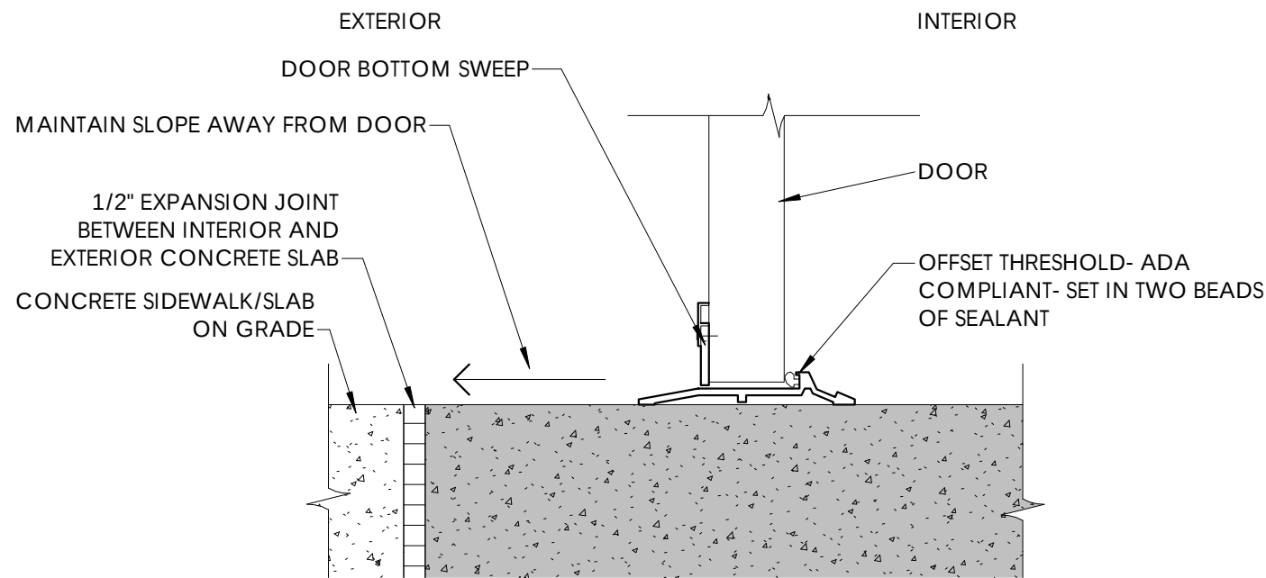
C3 A7.02 TYPICAL SWING DOOR SILL 3" = 1'-0"
