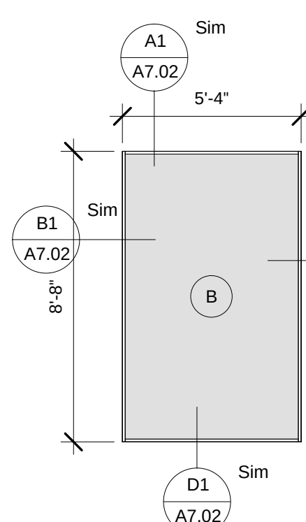
C9 A7.01 WINDOW TYPE B 1/4" = 1'-0"
