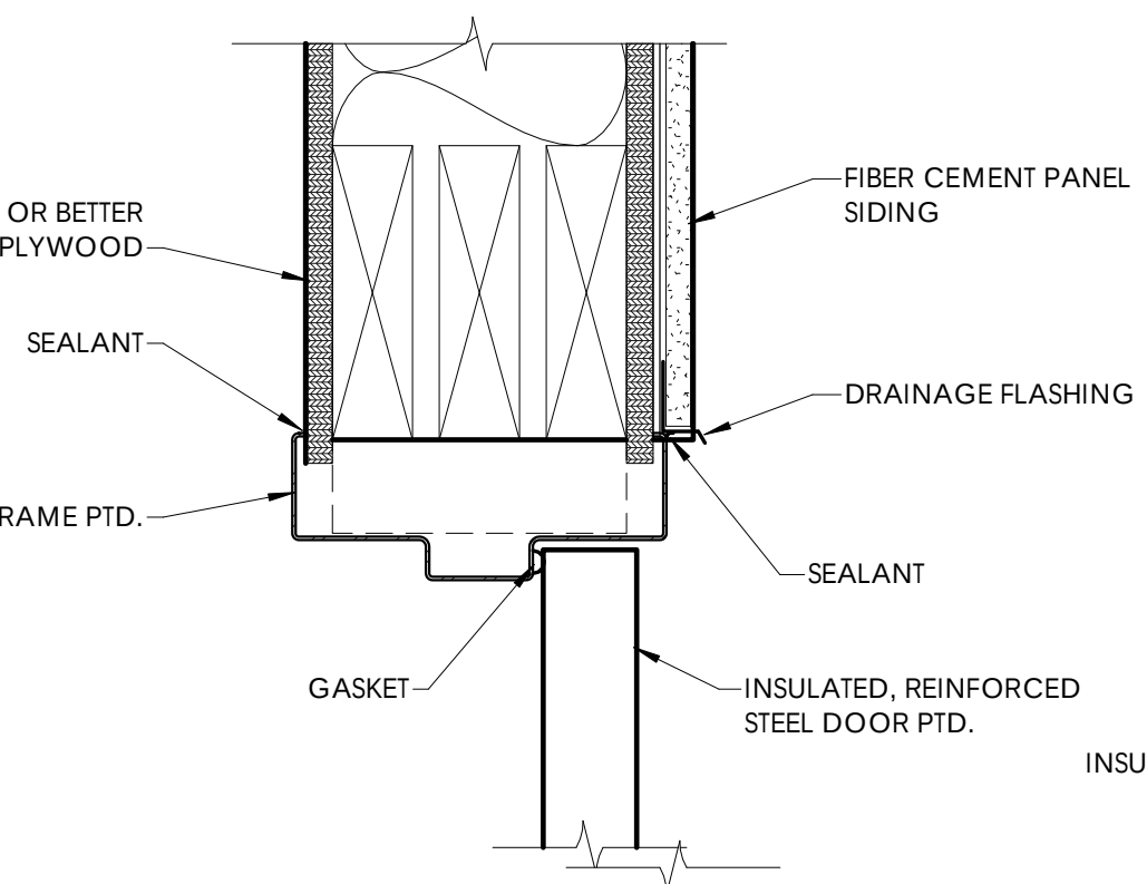
D4 A7.02 PATIO BAR DOOR HEAD 3" = 1'-0"
