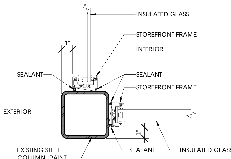
C1 A7.02 TYPICAL LOBBY WINDOW JAMB @ CORNER 3" = 1'-0"
