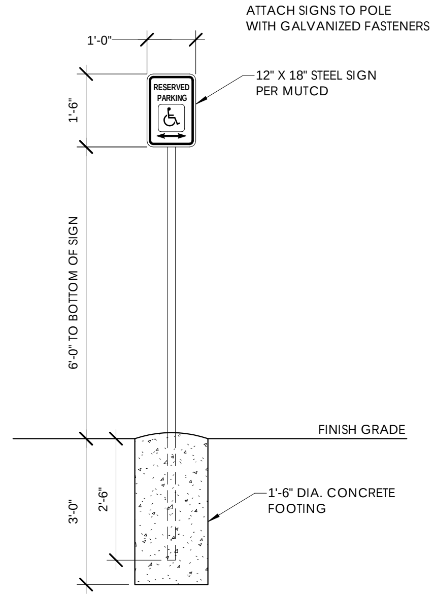
D5 A1.01 POLE MOUNTED SIGN 1/2" = 1'-0"
