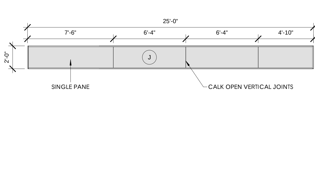
C1 A7.01 WINDOW TYPE J 1/4" = 1'-0"
