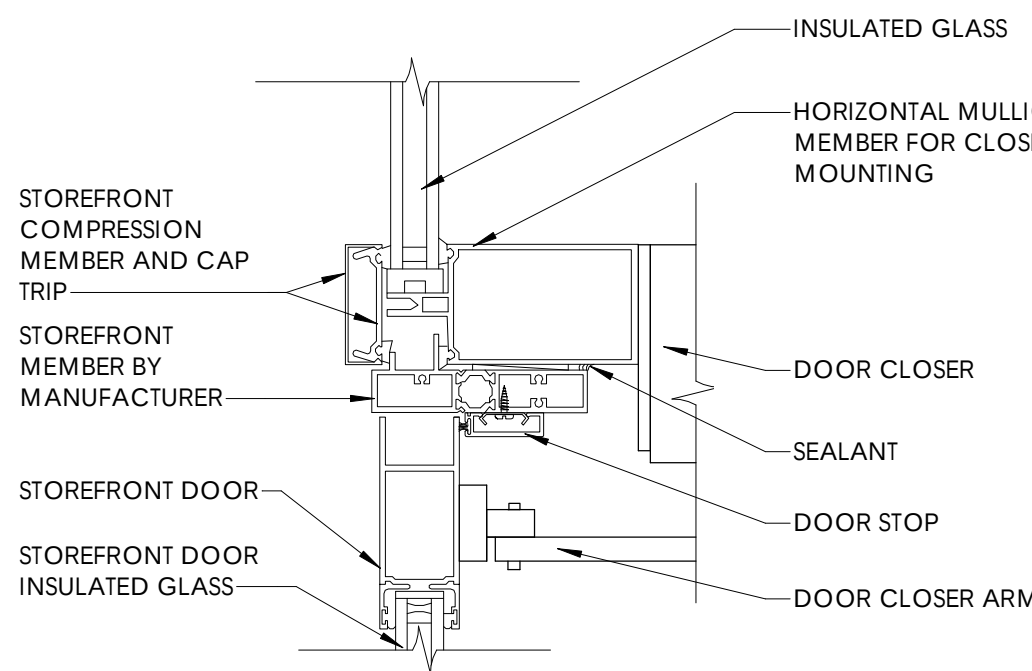
A2 A7.02 TYPICAL STOREFRONT DOOR HEAD 3" = 1'-0"
