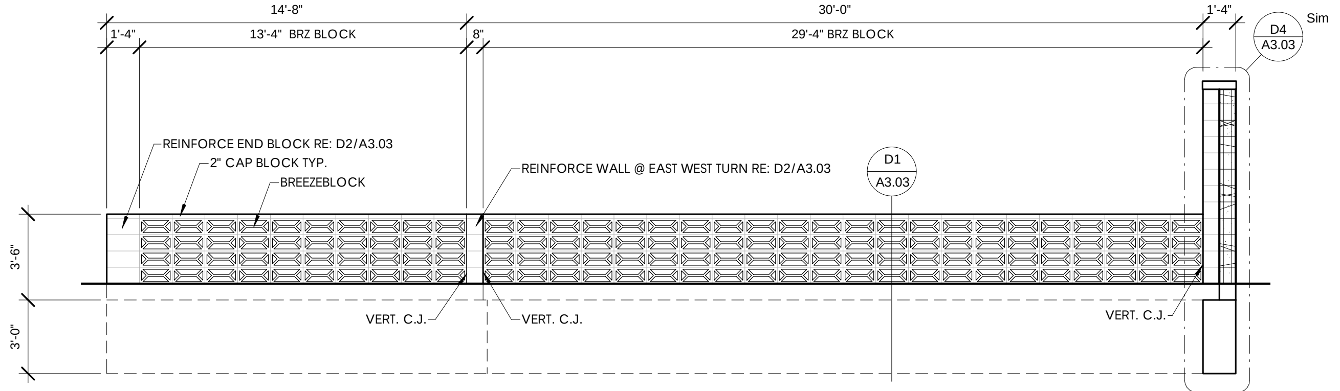
A2 A2.03 NORTH WALL 1/4" = 1'-0"
