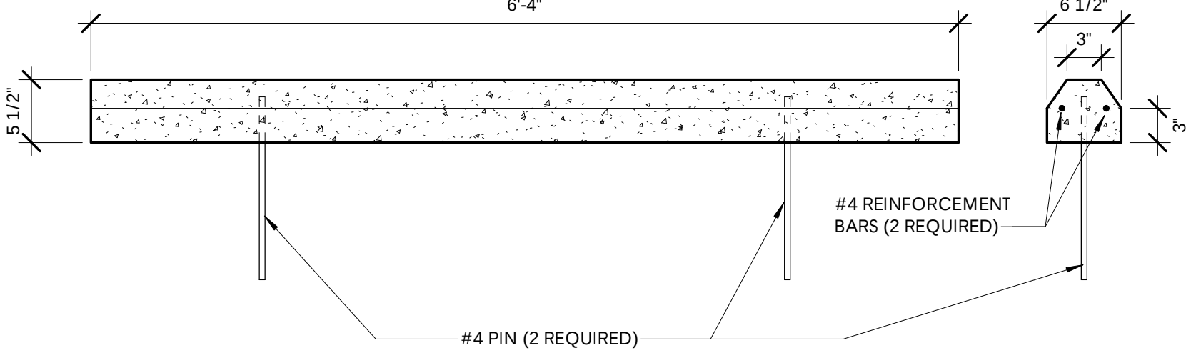
A2 A1.01 WHEEL STOP DETAIL 1" = 1'-0"
