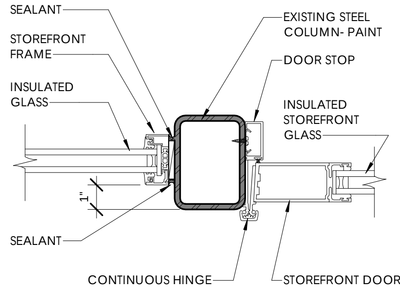
C2 A7.02 STOREFRONT DOOR JAMB @ HINGE 3" = 1'-0"
