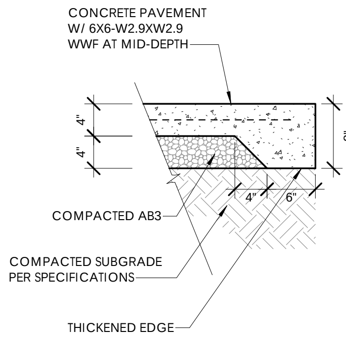
A4 A1.01 PAVEMENT DETAILS NOT TO SCALE
