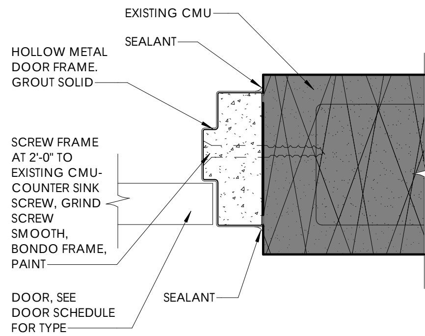
B3 A7.02 DOOR JAMB @ EXTERIOR BLOCK WALL 3" = 1'-0"
