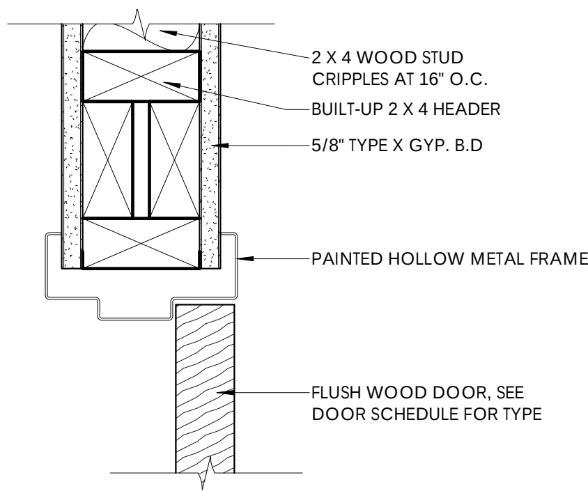
A4 A7.02 TYPICAL INTERIOR DOOR HEAD 3" = 1'-0"
