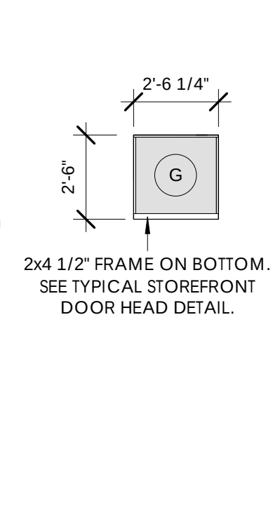
C4 A7.01 WINDOW TYPE G 1/4" = 1'-0"
