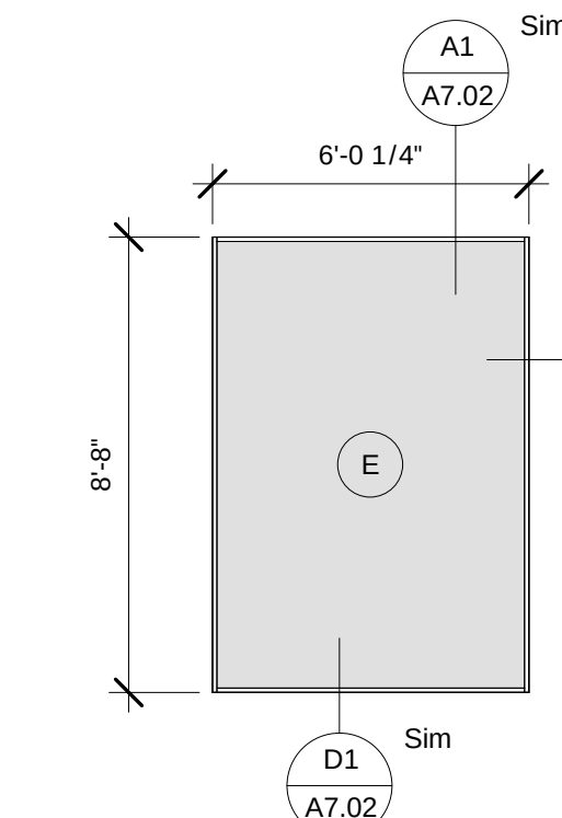
C6 A7.01 WINDOW TYPE E 1/4" = 1'-0"
