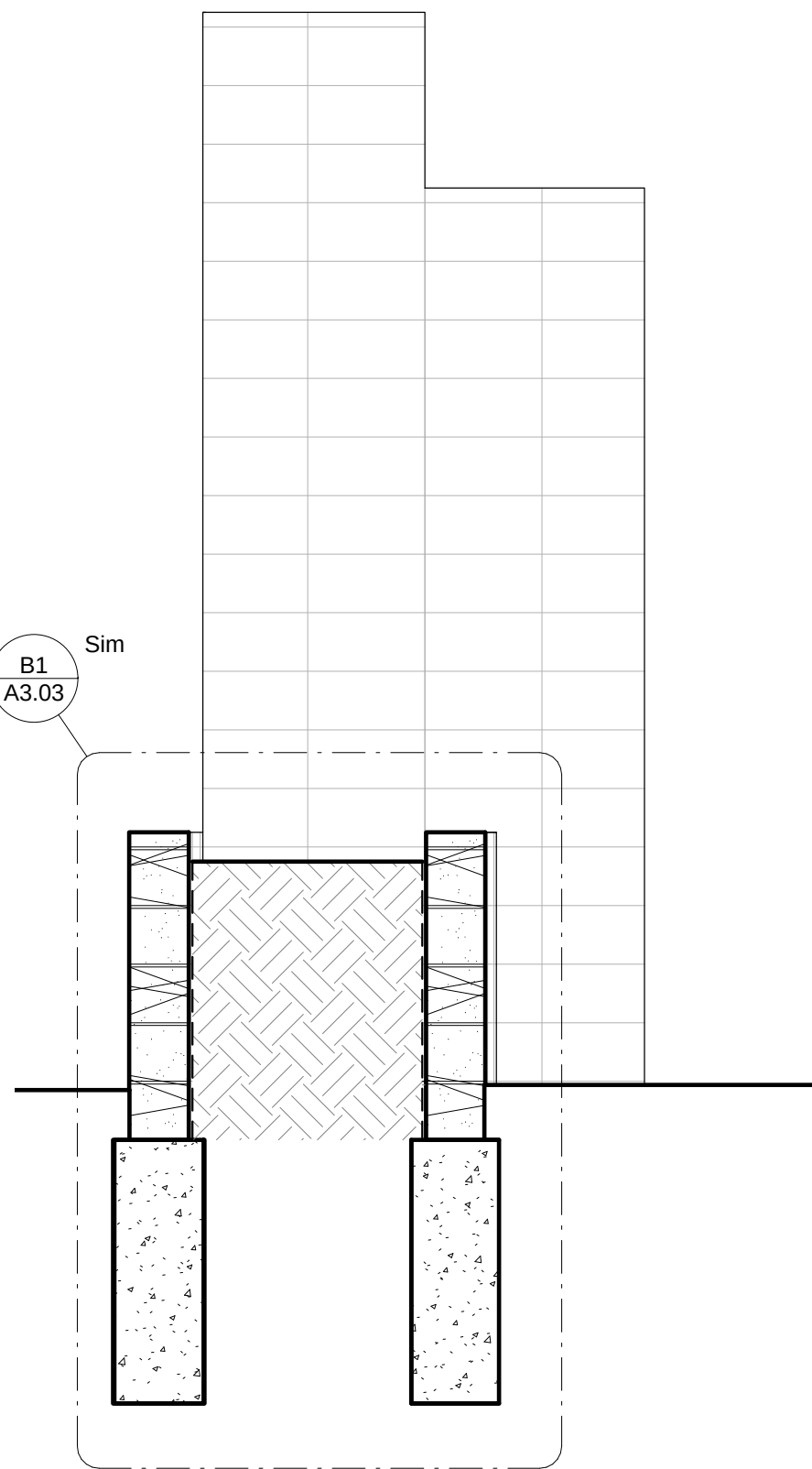
D5 A2.03 CORNER SIGN 1/2" = 1'-0"
