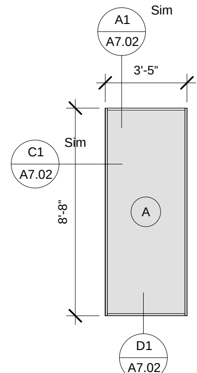
C10 A7.01 WINDOW TYPE A 1/4" = 1'-0"
