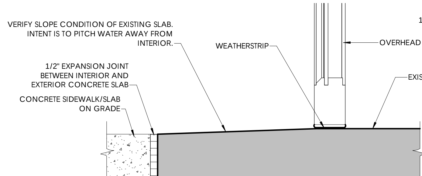
D5 A7.02 OVERHEAD DOOR SILL 3" = 1'-0"
