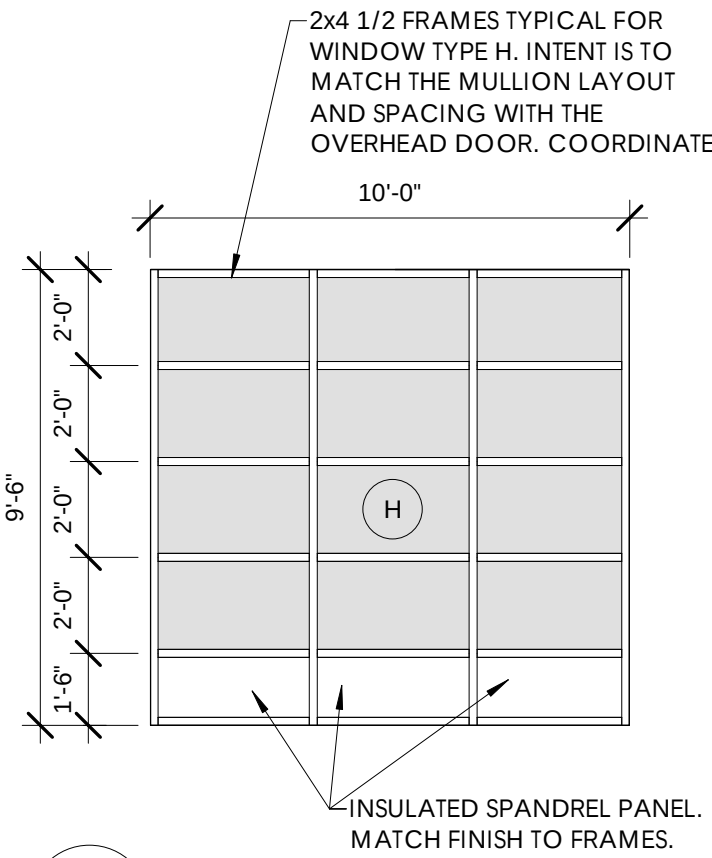
C3 A7.01 WINDOW TYPE H 1/4" = 1'-0"
