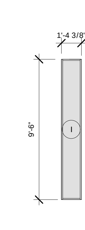
C2 A7.01 WINDOW TYPE I 1/4" = 1'-0"
