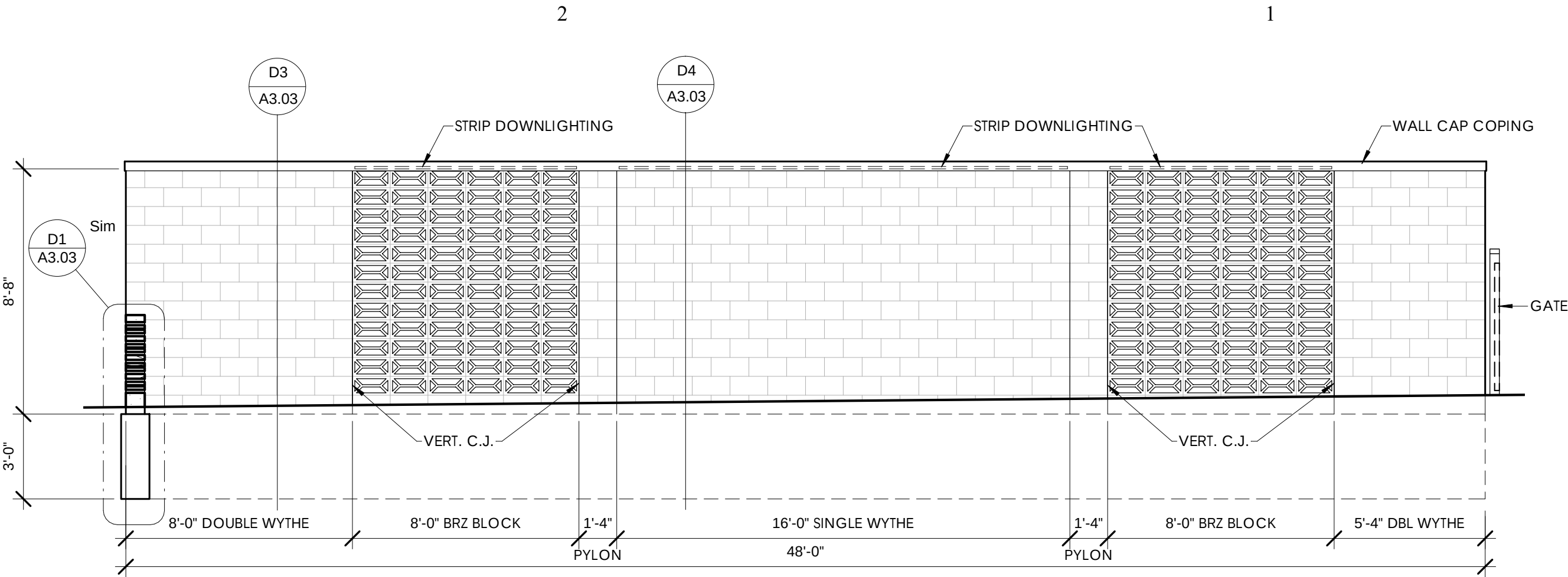
A2 A2.03 NORTH WALL 1/4" = 1'-0"
