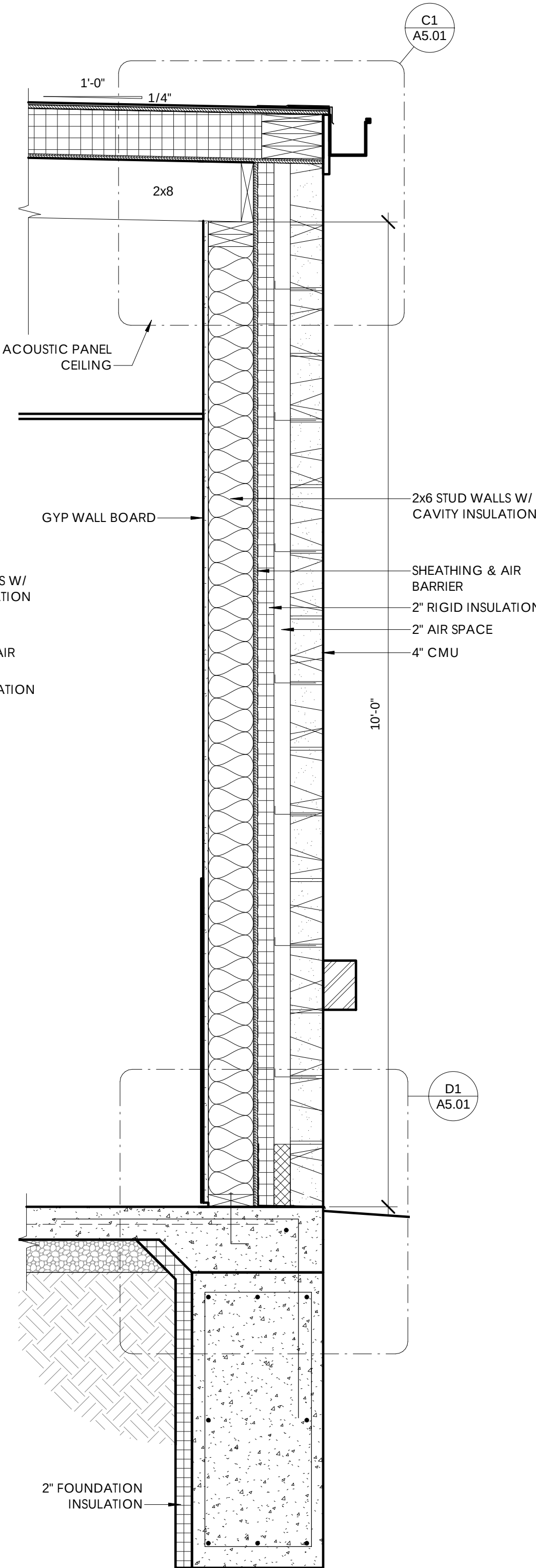
D2 A3.02 TYPICAL ADDITION EAST WALL SECTION 1" = 1'-0"
