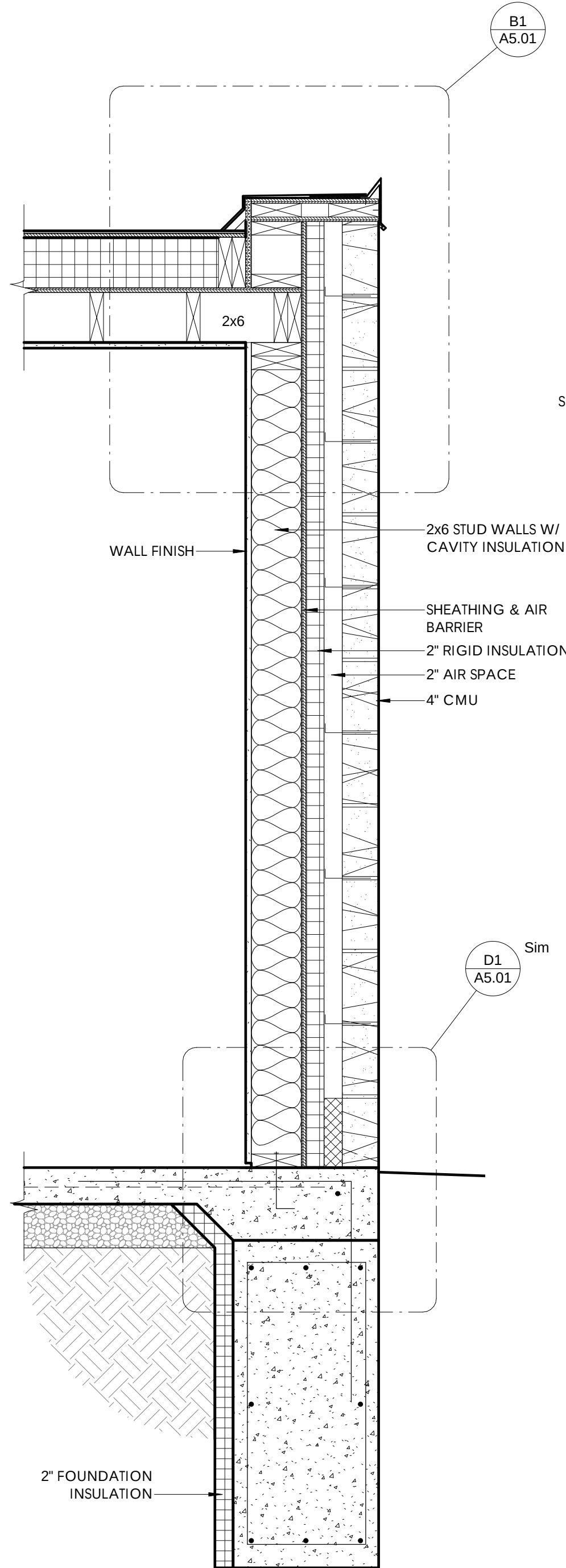
D4 A3.02 WALL SECTION @ SOUTH ADDITION WALL 1" = 1'-0"
