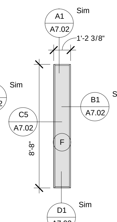
C5 A7.01 WINDOW TYPE F 1/4" = 1'-0"
