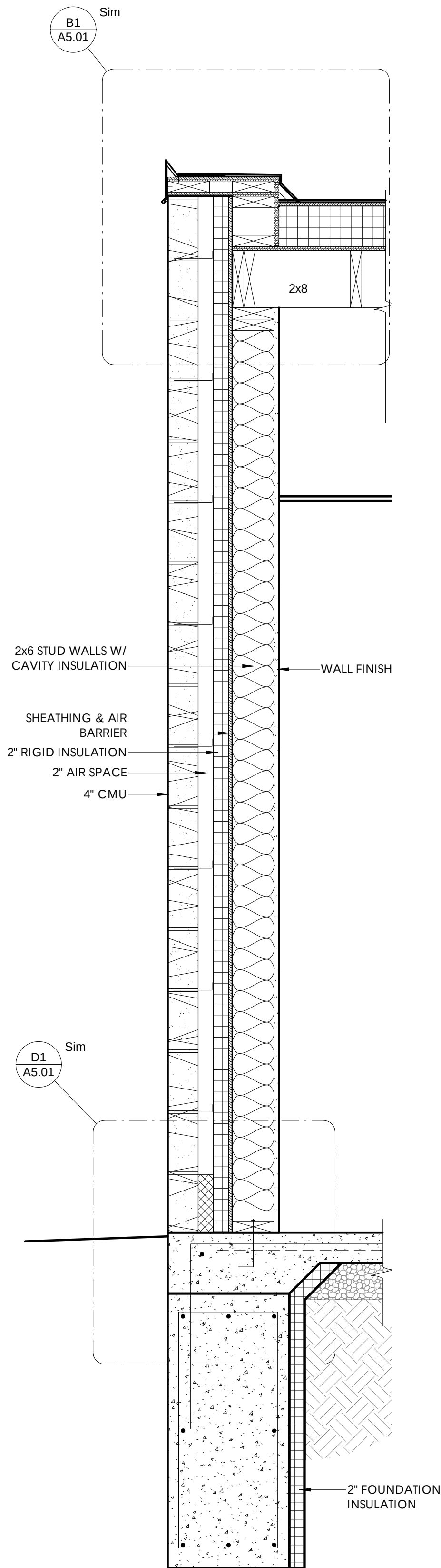
D6 A3.02 WALL SECTION @ NORTH ADDITION WALL 1" = 1'-0"
