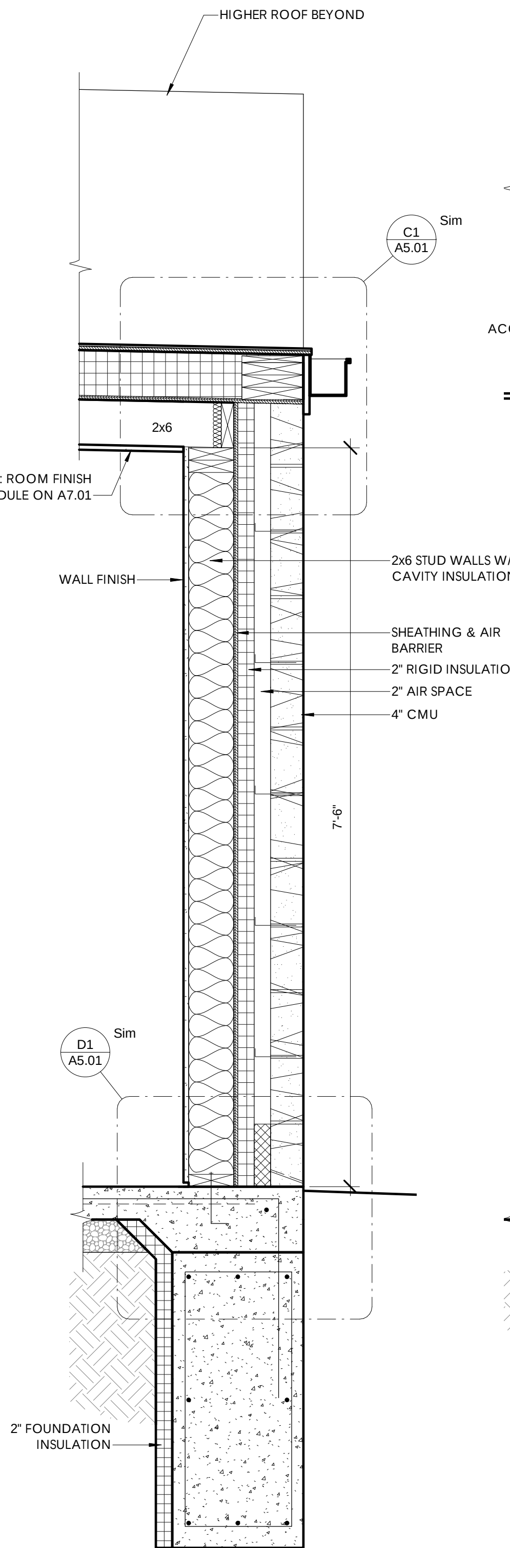
D3 A3.02 WALL SECTION @ LOWER WALL ELEVATION 1" = 1'-0"
