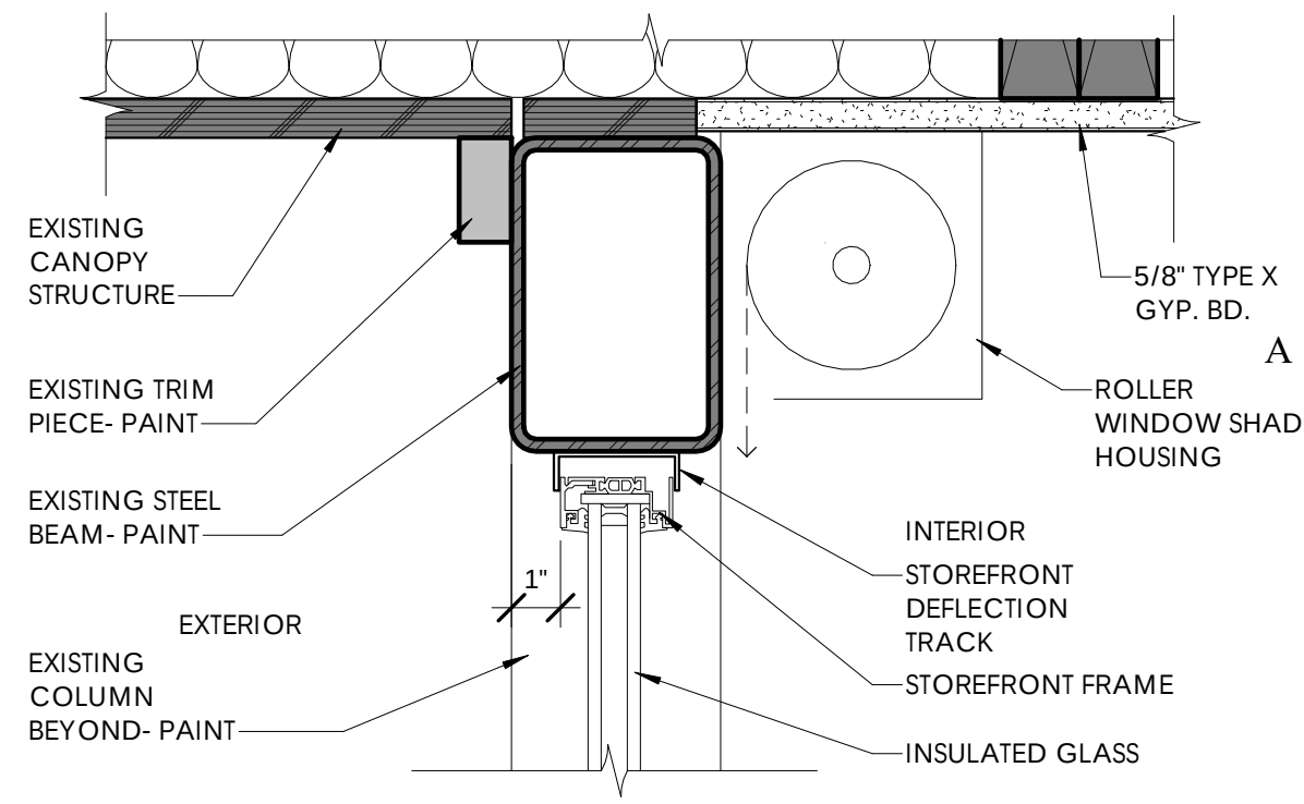
A1 A7.02 TYPICAL LOBBY WINDOW HEAD 3" = 1'-0"
