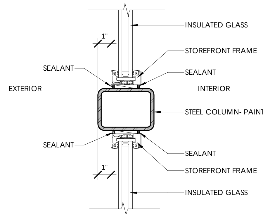
B1 A7.02 TYPICAL LOBBY WINDOW JAMB 3" = 1'-0"
