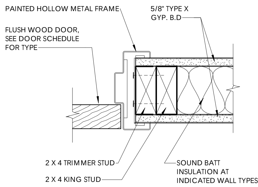
B4 A7.02 TYPICAL INTERIOR DOOR JAMB 3" = 1'-0"
