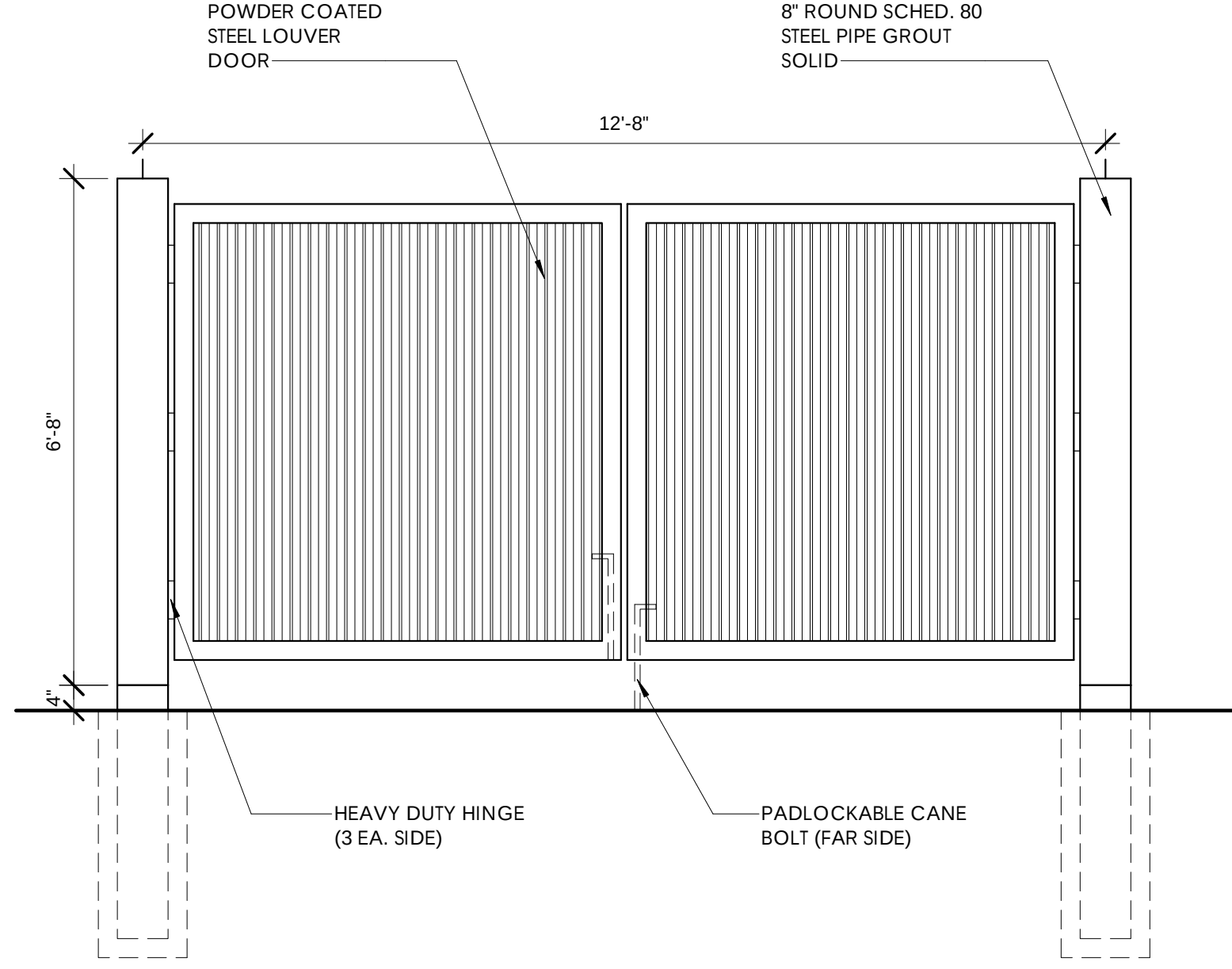
C4 A1.01 ELEVATION @ TRASH ENCLOSURE GATE 1/2" = 1'-0"
