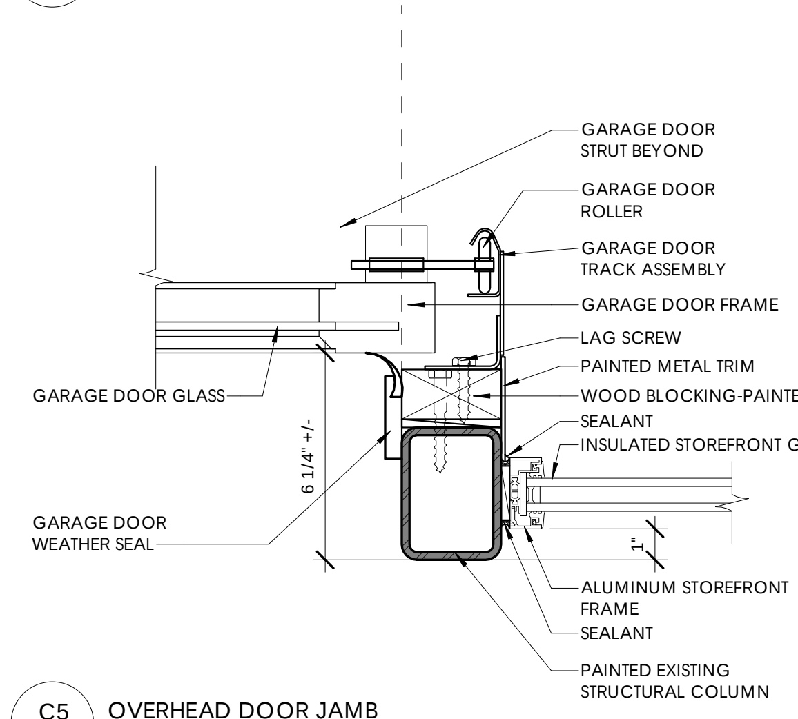
C5 A7.02 OVERHEAD DOOR JAMB 3" = 1'-0"
