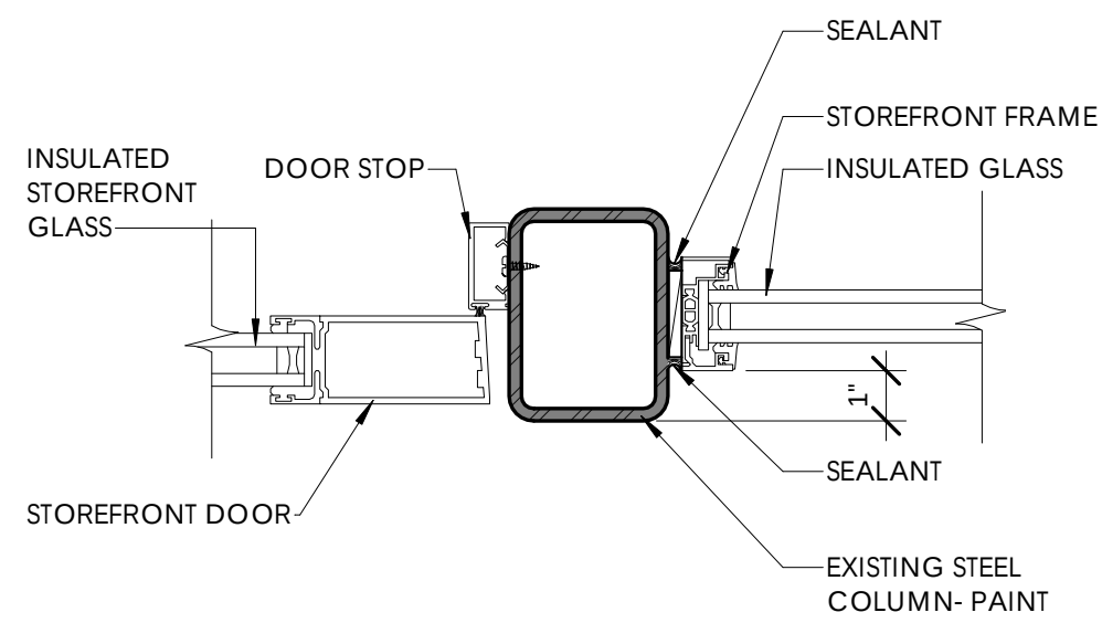
B2 A7.02 STOREFRONT DOOR JAMB 3" = 1'-0"
