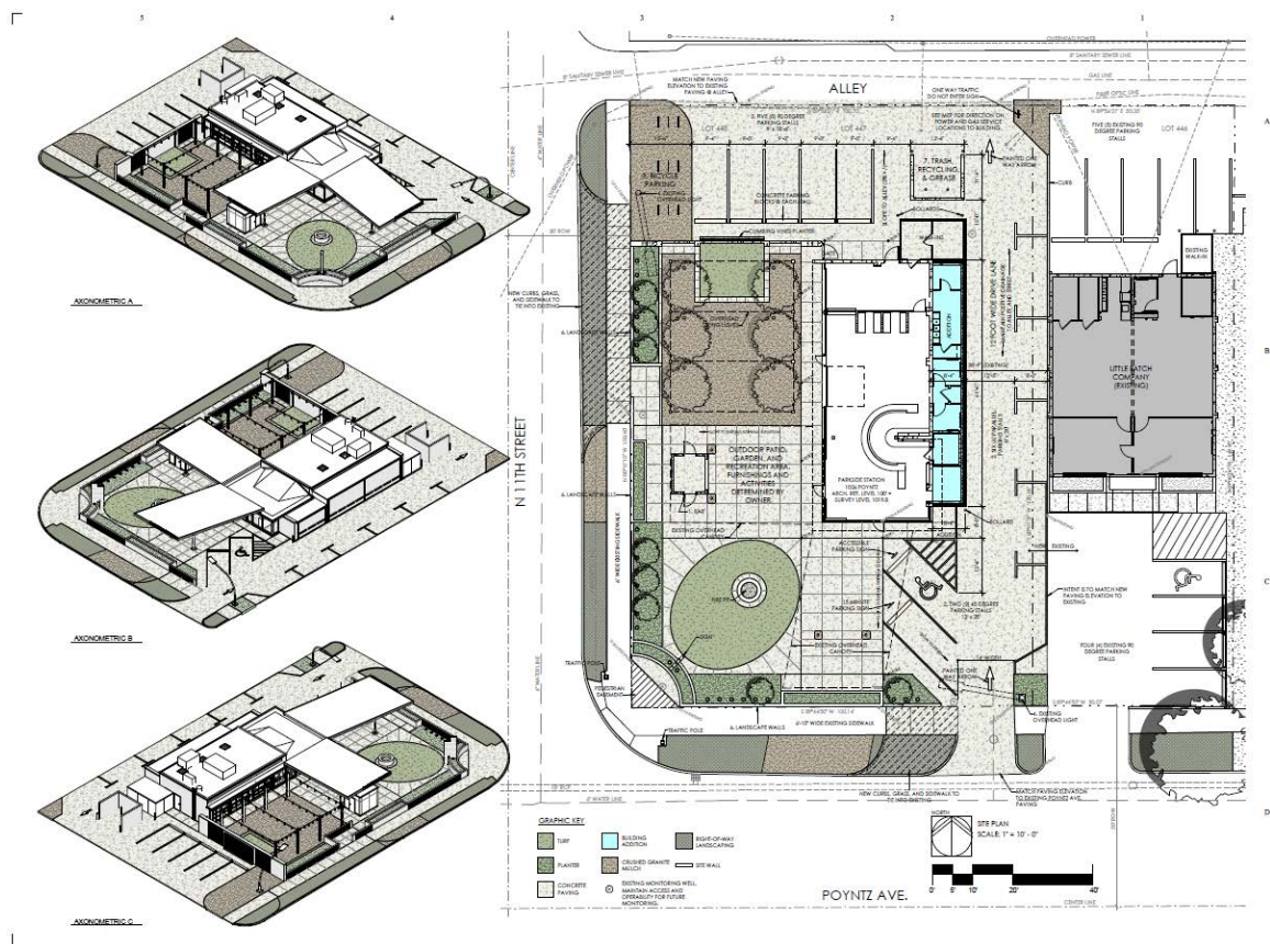
Figure 4: Site Plan of Proposed, BBN Architects.
