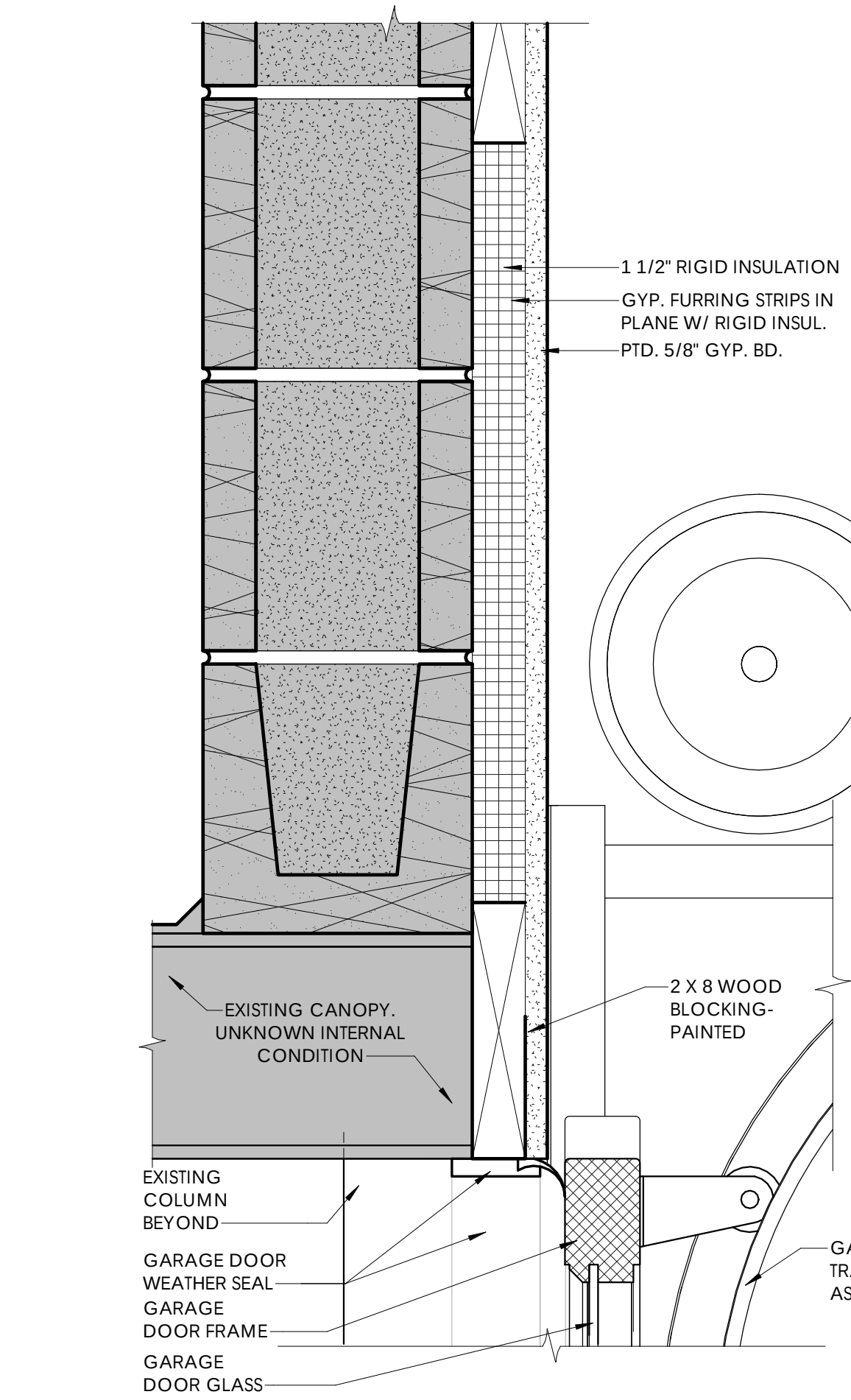
B5 A7.02 OVERHEAD DOOR HEAD 3" = 1'-0"
