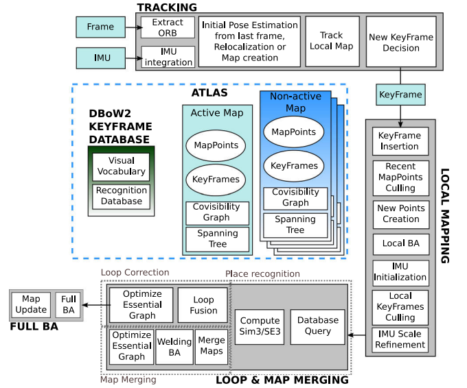
Fig. 1. Main system components of ORB-SLAM3.
