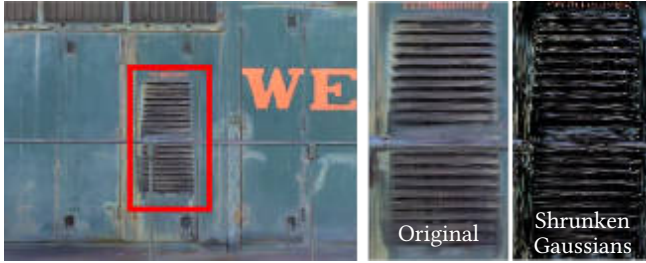
Fig. 3. We visualize the 3D Gaussians after optimization by shrinking them 60% (far right). This clearly shows the anisotropic shapes of the 3D Gaussians that compactly represent complex geometry after optimization. Left the actual rendered image.
