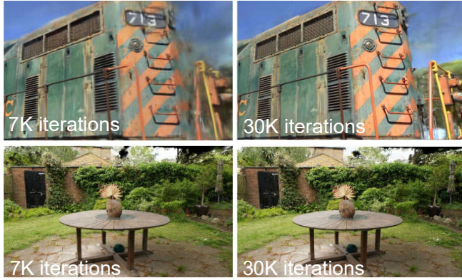
Fig. 6. For some scenes (above) we can see that even at 7K iterations (~5min for this scene), our method has captured the train quite well. At 30K iterations (~35min) the background artifacts have been reduced significantly. For other scenes (below), the difference is barely visible; 7K iterations (~8min) is already very high quality.
