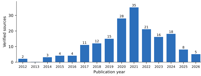
Fig. 11. Temporal distribution of the 182 verified primary sources by publication year (2012–2026). The peak in 2020–2024 coincides with the parallel maturation of RGB-D fusion, foundation-model monocular depth, and end-to-end detection.
