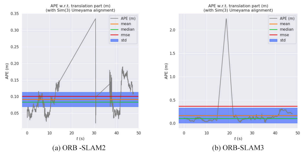
Figure 12. The ATE variation over time on the Rgbid_kidnap public dataset. The gray line represents the ATE curve over time; the orange line indicates the mean ATE ; the green line represents the median ATE ; the red line denotes the RMSE of the ATE ; and the purple shaded area indicates the standard deviation of the ATE .
