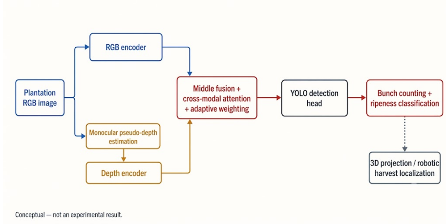
Figure 10: The proposed — and explicitly conceptual, not yet validated — RGB-D pipeline for oil-palm FFB perception: a plantation RGB image feeds an RGB encoder and, in parallel, a monocular pseudo-depth branch; quality-aware fusion feeds a real-time detector; per-instance maturity, an instance-constrained depth sample, and pose-based temporal association then produce a de-duplicated bunch inventory. Every stage corresponds to an ablation in the agenda below.
