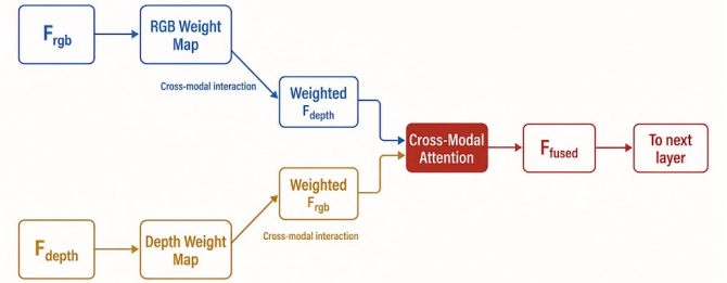
Fig. 7. The cross-modal attention mechanism that recurs across the strongest RGB-D methods (e.g. SA-Gate, CIR-Net, CMX): each modality generates a weighting map that gates the other before fusion, so a faulty depth measurement can be suppressed rather than allowed to contaminate the joint representation.
