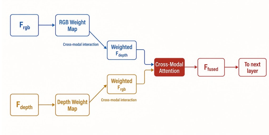
Figure 7: The cross-modal attention mechanism that recurs across the strongest RGB-D methods (e.g. SA-Gate, CIR-Net, CMX): each modality generates a weighting map that gates the other before fusion, so a faulty depth measurement can be suppressed rather than allowed to contaminate the joint representation.
