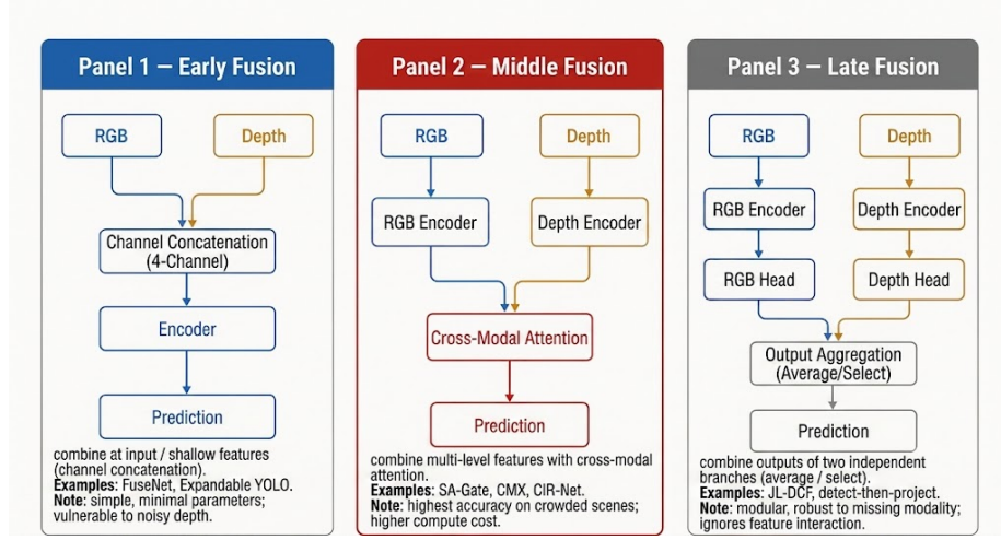
Figure 6: The three fusion locations that structure the RGB-D literature. Early fusion concatenates colour and depth at the input (e.g. FuseNet, Expandable YOLO); middle/feature fusion learns modality-specific representations before exchanging them at selected scales; late fusion combines predictions and supports an explicit RGB fallback.
